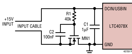
Figure 4. Input Soft Connect Circuit
