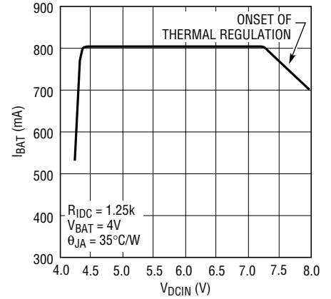
Charge Current vs Supply Voltage
