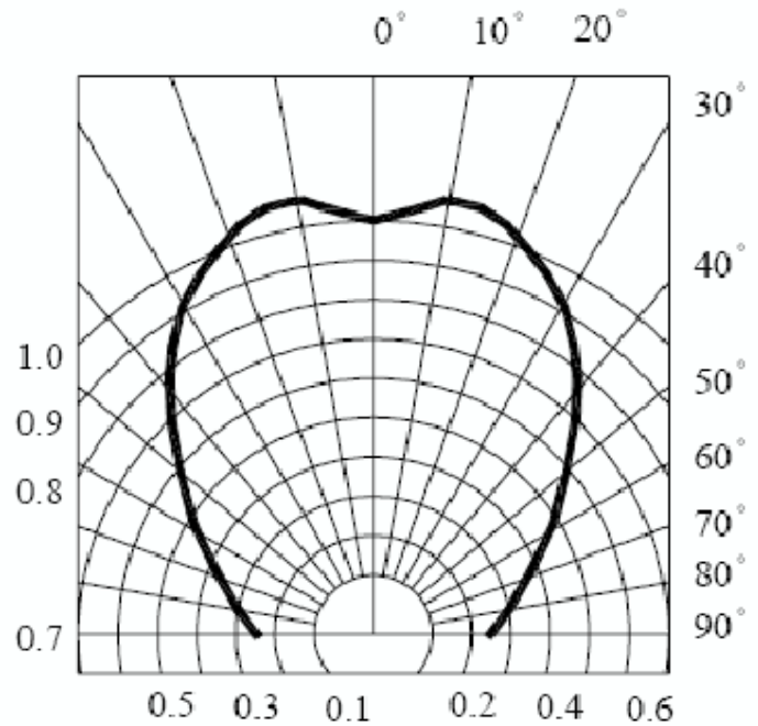
RADIATION DIAGRAM
