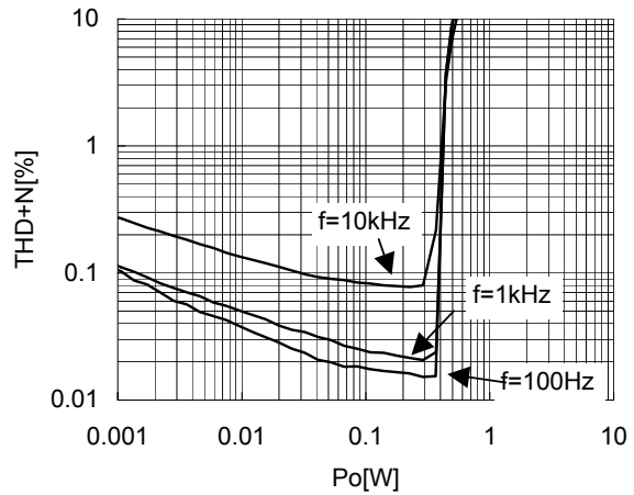
THD+N vs Po(BTL) V_+ = 3.3V , V_{ol} = 0dB , R_L = 8\Omega , T_a = 25^\circ C InternalGain, BW=22Hz to 30kHz
