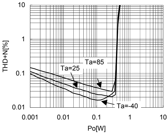
THD+N vs Po(BTL) V_+ = 3.3V , f = 1kHz , V_{ol} = 0dB , R_L = 8\Omega InternalGain, BW=400Hz to 30kHz
