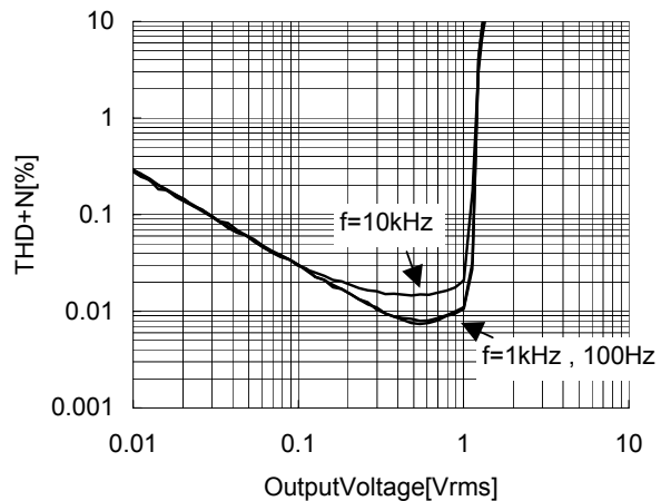
THD+N vs OutputVoltage(MonOut) V_+ = 3.3V , R_L = 100k\Omega , T_a = 25^\circ C BW=22Hz to 30kHz
