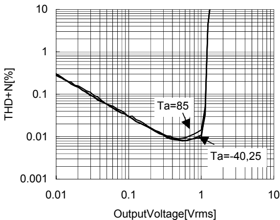
THD+N vs OutputVoltage(MonOut) V_+ = 3.3V , f = 1kHz , R_L = 100k\Omega BW=400Hz to 30kHz
