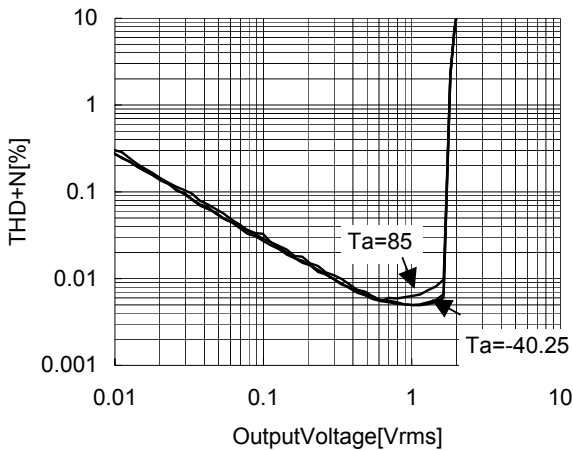
THD+N vs OutputVoltage(MonOut) V_+ = 5V , f = 1kHz , R_L = 100k\Omega BW=400Hz to 30kHz
