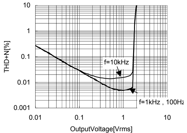
THD+N vs OutputVoltage(MonOut) V_+ = 5V , R_L = 100k\Omega , T_a = 25^\circ C BW=22Hz to 30kHz
