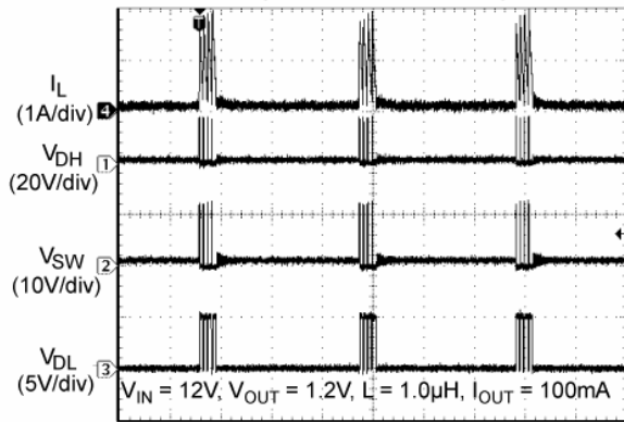
Switching Waveform (Discontinuous Mode)
