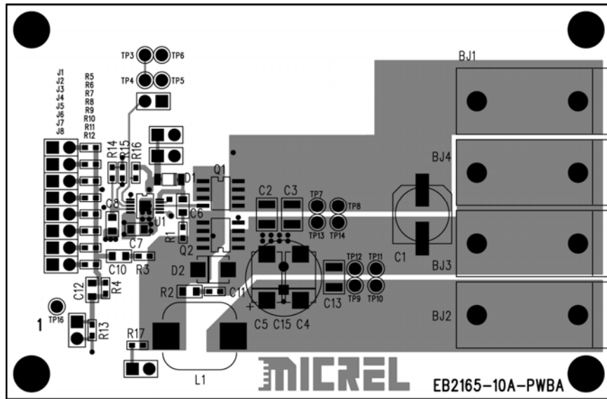
Figure 11. MIC2165 10A Evaluation Board Top Layer
