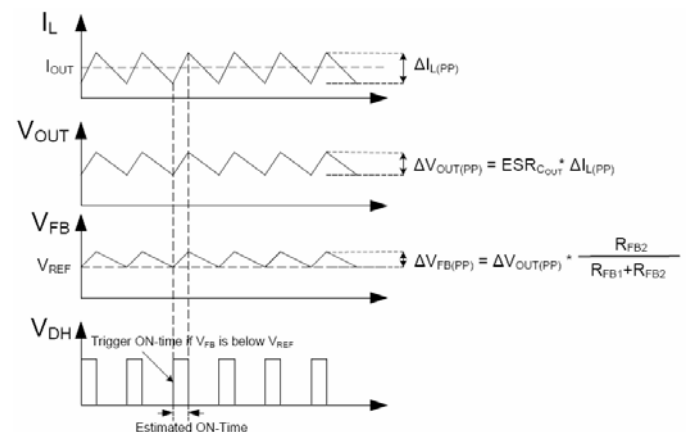
Figure 2. MIC2165 Control Loop Timing (Continuous Mode)
