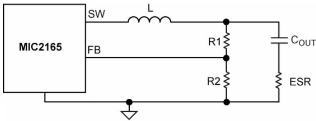
Figure 9a. \frac{R2}{R1+R2} \times \Delta V_{OUT} > 20mV
