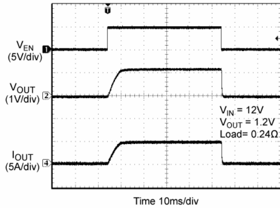
Power-Up/Power-Down
