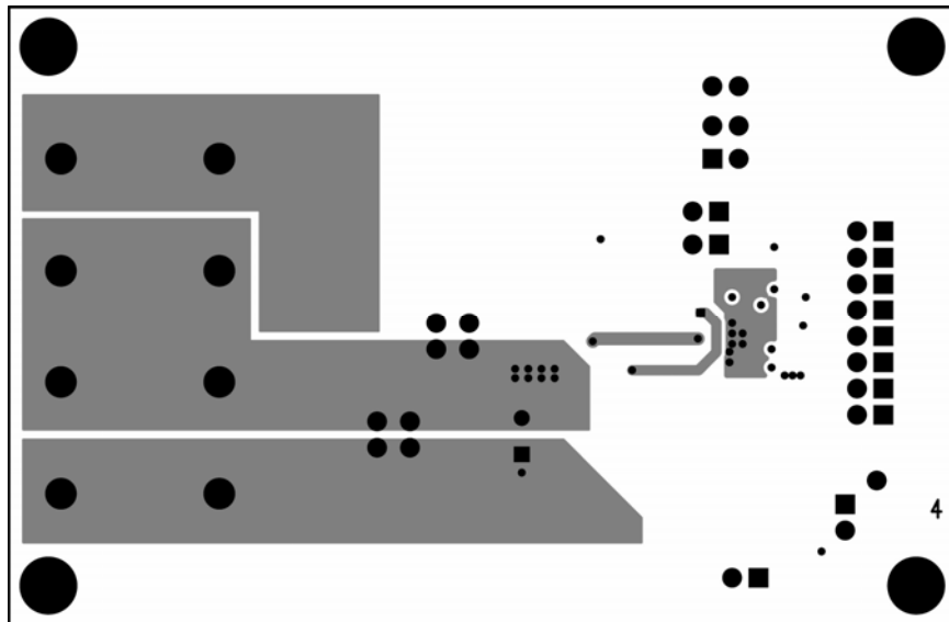
Figure 12. MIC2165 10A Evaluation Board Bottom Layer
