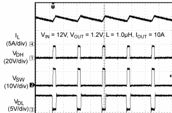
Switching Waveform (Continuous Mode)
