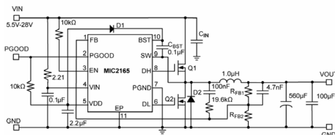
MIC2165 Adjustable Output 600kHz Buck Converter
