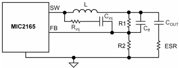
Figure 9c. \Delta V_{OUT} < 20mV
