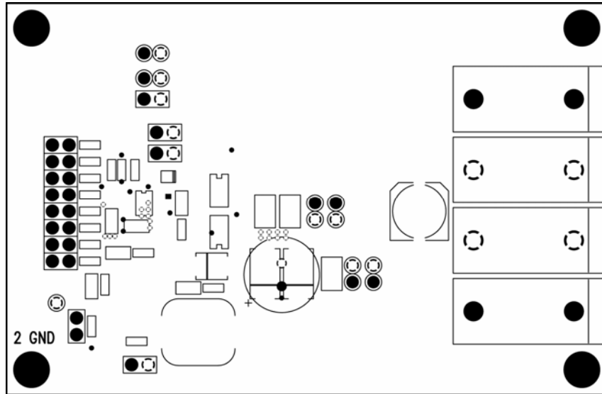
Figure 13. MIC2165 10A Evaluation Board Mid-Layer 1 (GND Plane)
