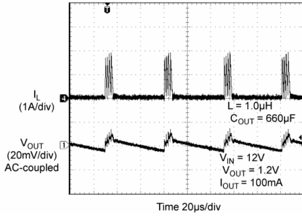
Output Voltage Ripple (Discontinuous Mode)
