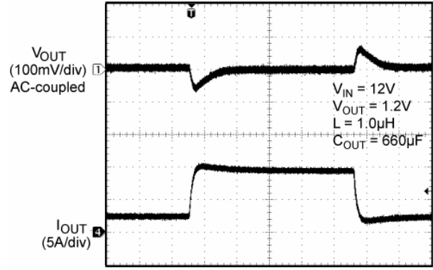
Load Transient (2.5A to 10A) Continuous Mode
