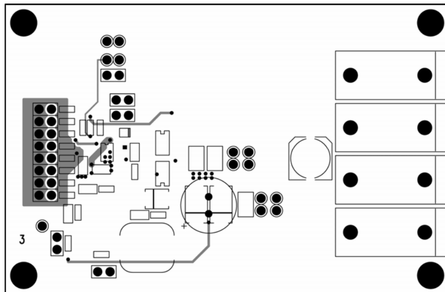
Figure 14. MIC2165 10A Evaluation Board Mid-Layer 2
