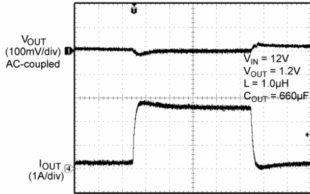
Load Transient (100mA to 2.5A) Discontinuous Mode to Continuous Mode
