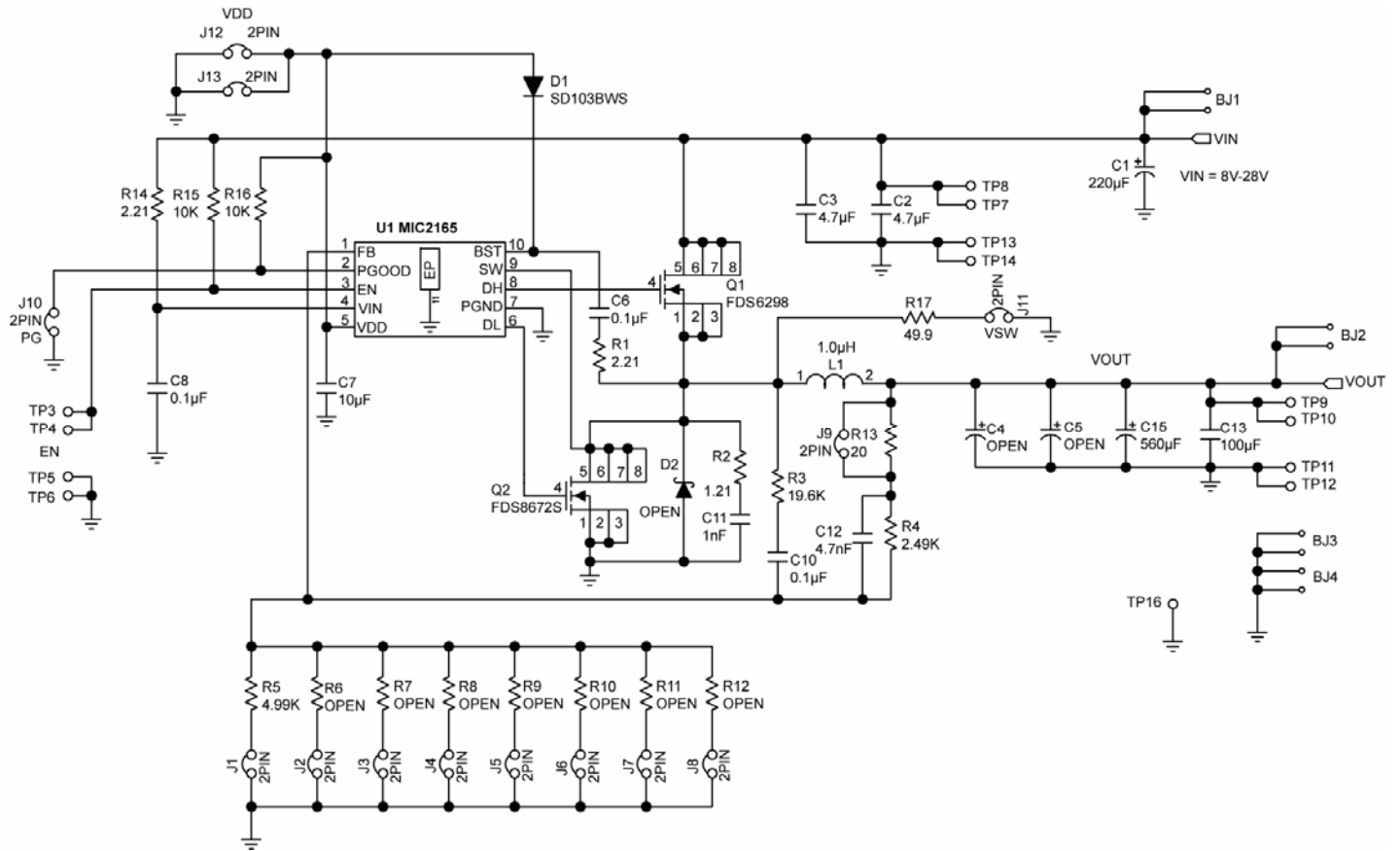
Figure 10. Schematic of MIC2165 8-24 VIN to 1.2 VOUT/10A Evaluation Board
