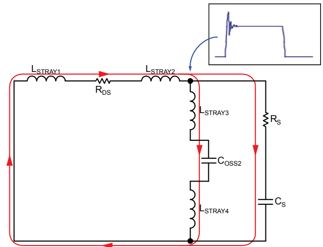
Figure 8. Snubber Circuit
