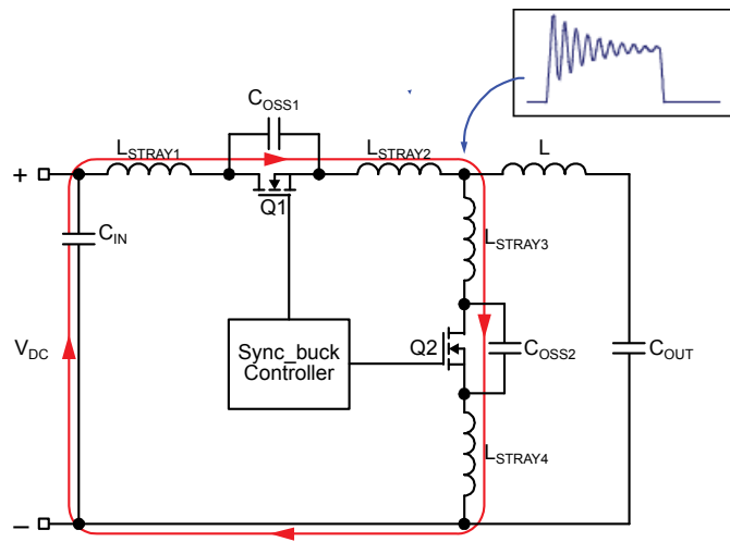
Figure 7. Output Parasitics
