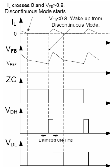
Figure 4. MIC2165 Control Loop Timing (Discontinuous Mode)
