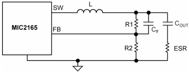
Figure 9b. \frac{R2}{R1+R2} \times \Delta V_{OUT} < 20mV and \Delta V_{OUT} > 20mV
