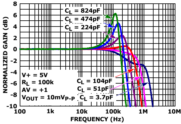
FIGURE 21. GAIN vs FREQUENCY vs C_L
