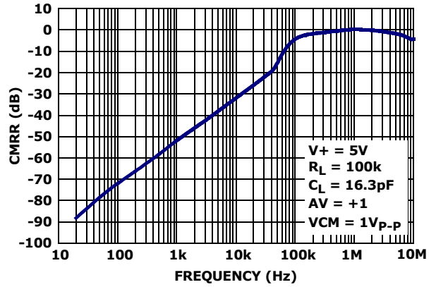
FIGURE 22. CMRR vs FREQUENCY, V_S = 5V
