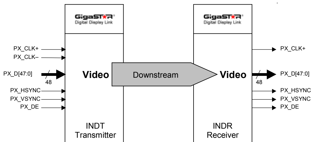
Figure 1.2: Pixel Interface
