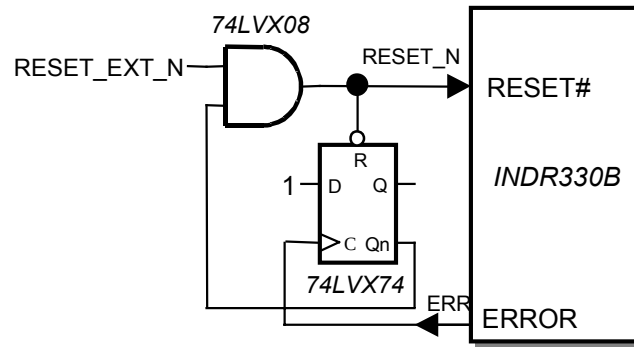
Figure 2.3: Auto-Reset Circuitry
