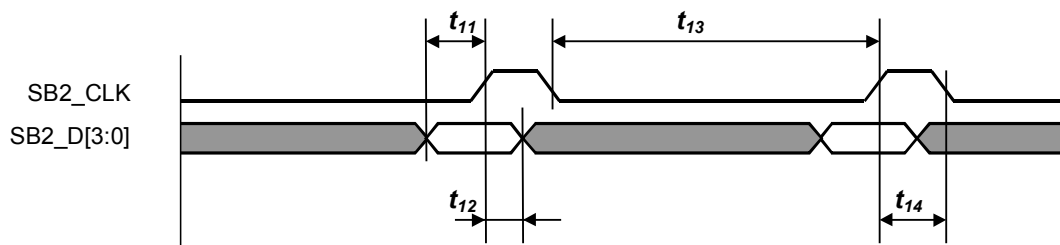
Figure 3.8: Tx Sideband Data Interface; Low Speed Downstream
