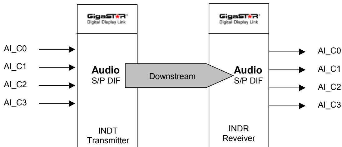
Figure 1.7: Audio Interface
