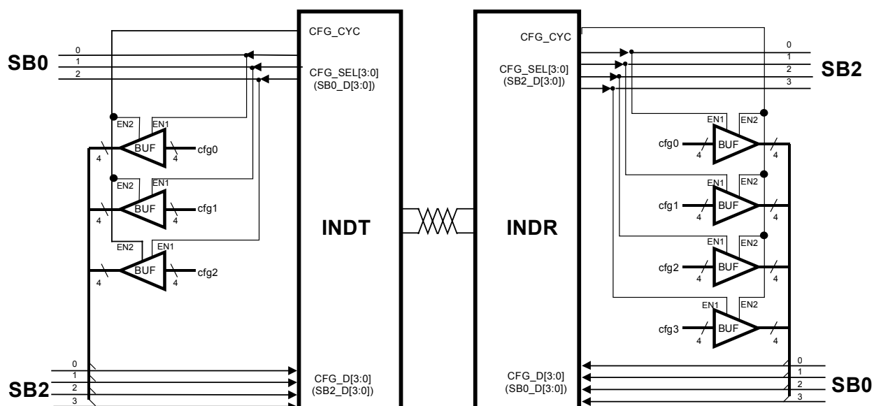
Figure 2.1: Configuration Logic
