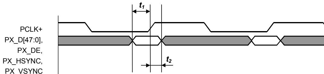
Figure 3.4: Pixel Interface Timing Diagram At Rising Edge At Tx
