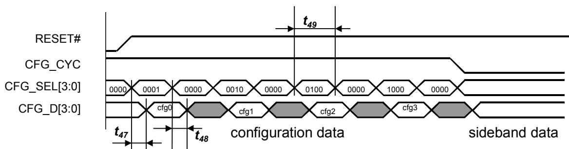
Figure 3.16: Configuration Interface Timing
