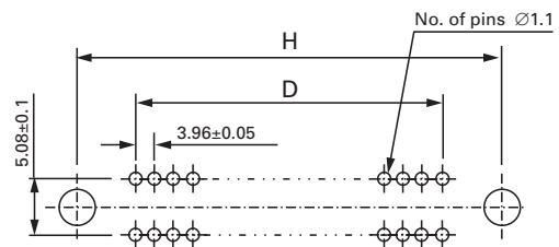
Top View from Socket
