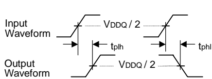
Fig.2 Tdly measurement
