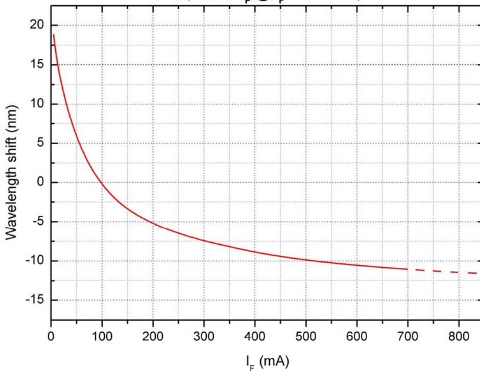
Typical wavelength shift vs. forward current (rel. to \lambda_p @ I_F = 100 \text{ mA} )
