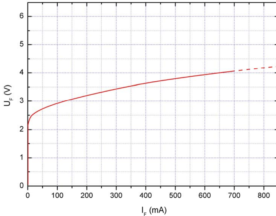
Forward voltage vs. forward current (typical)
