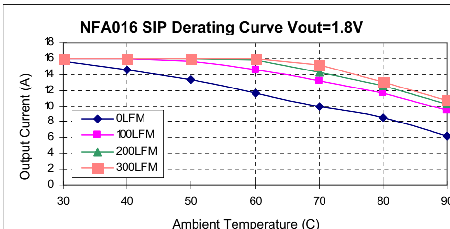
Fig 9. SIP Power Derating vs Output Current for 12Vin 1.8V Out.
