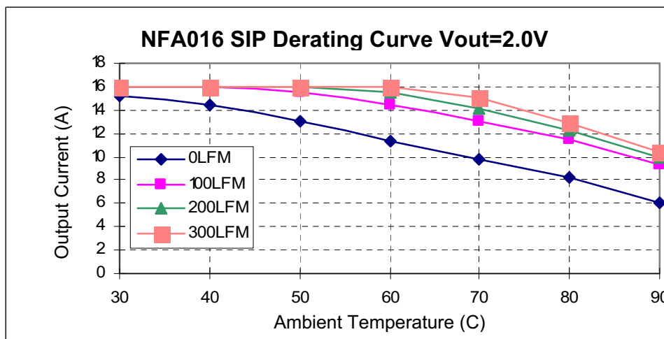
Fig 11. SIP Power Derating vs Output Current for 12Vin 2.0V Out.
