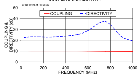
LRDC-10-2-75J COUPLING & DIRECTIVITY
