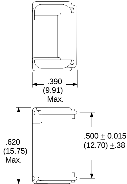
Physical Dimensions inches (mm)
