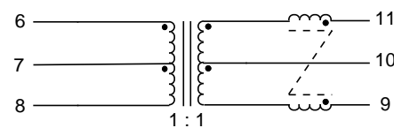
Receive Channel
