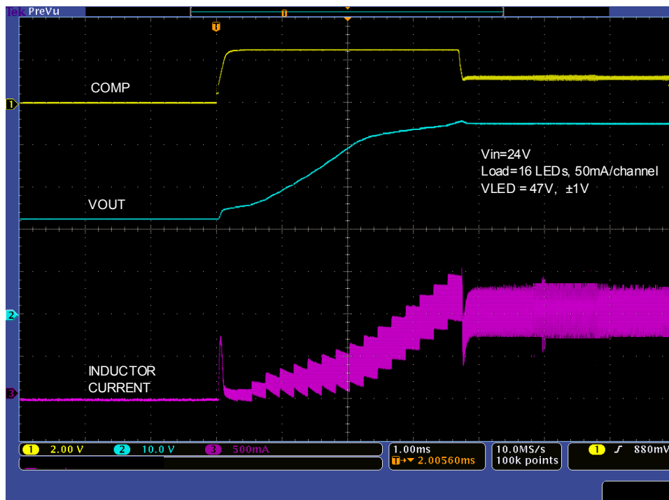
Figure 13. Boost Soft Start
