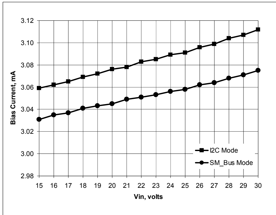
Figure 12. Bias Current vs Input Voltage (Sleep Mode)
