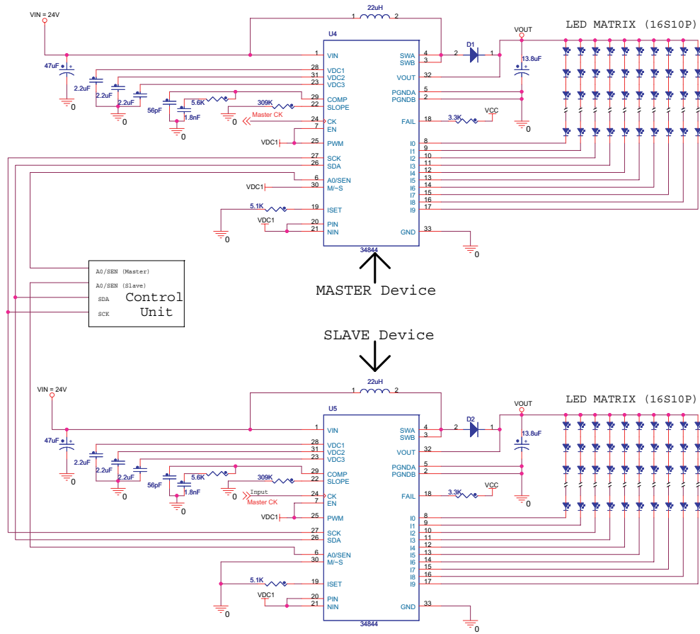
Figure 21. Master - Slave Connection
