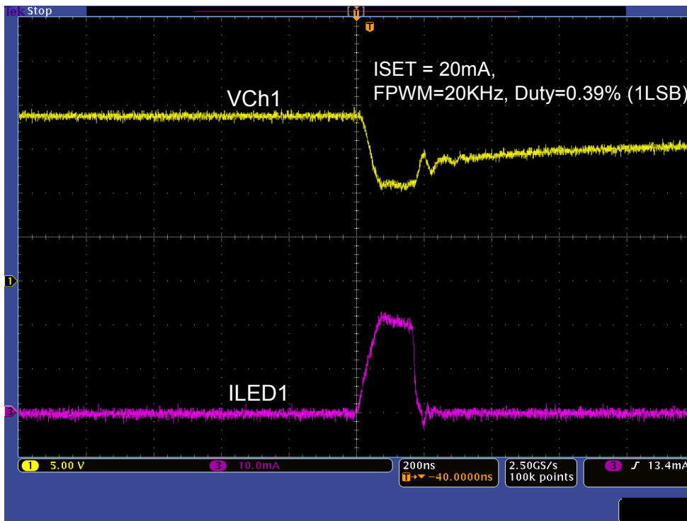
Figure 17. Low Duty Dimming Operation Waveforms (FPWM=20 kHz, 1LSB)
