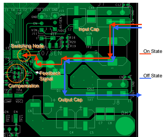
Figure 23. Feedback Signal Tracing
