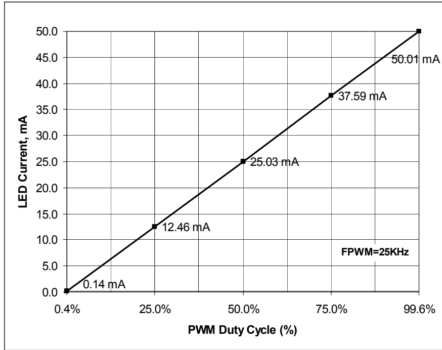
Figure 10. PWM Dimming Linearity
