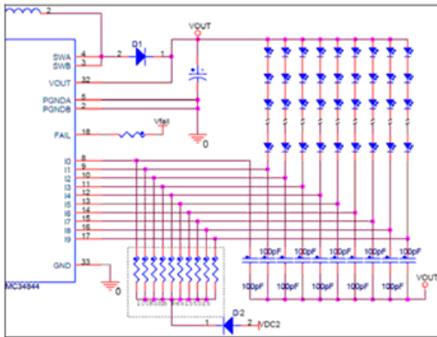
Figure 6. Resistor/Diode placement for multiple open circuit detection
