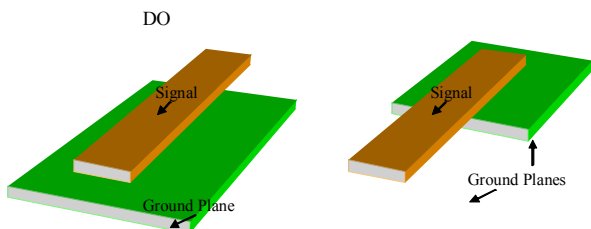
Figure 22. Recommended shielding for critical signals.
