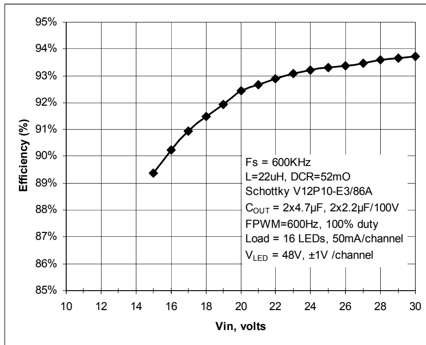
Figure 8. Boost efficiency vs Input Voltage
