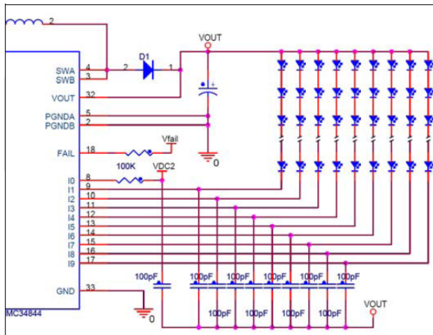
Figure 5. Single Channel Disconnect Circuit.
