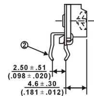
SUGGESTED PWB LAYOUT – STYLES K.P.W
