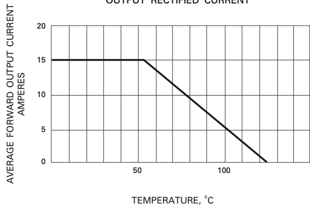
Fig.2 - DERATING CURVE FOR OUTPUT RECTIFIED CURRENT
