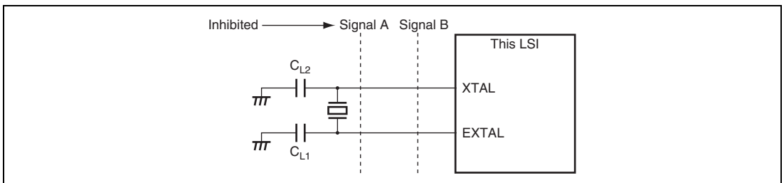
Figure 24.7 Note on Board Design for Oscillation Circuit
