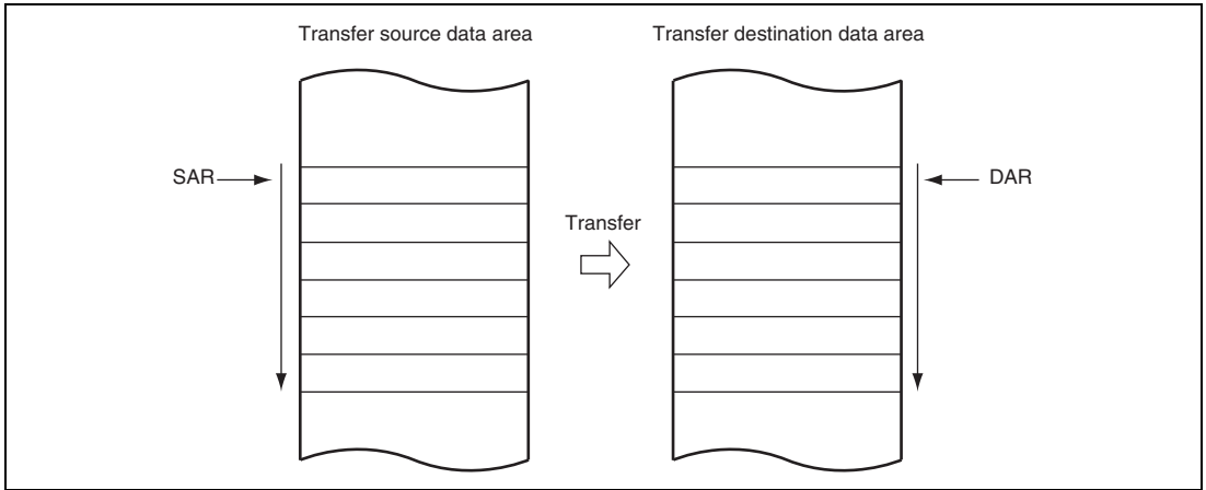
Figure 11.7 Memory Map in Normal Transfer Mode
