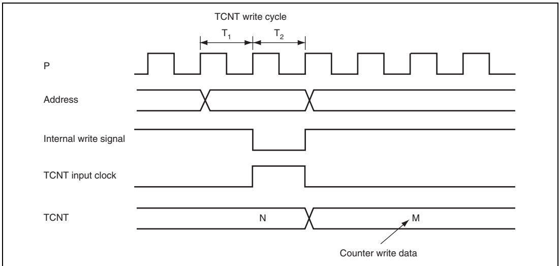
Figure 16.5 Conflict between TCNT Write and Increment
