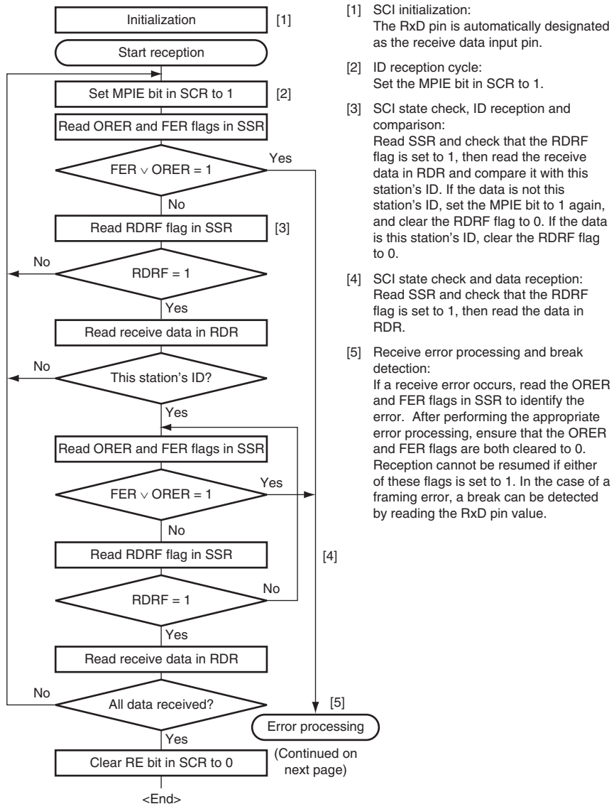
Figure 17.16 Sample Multiprocessor Serial Reception Flowchart (1)
