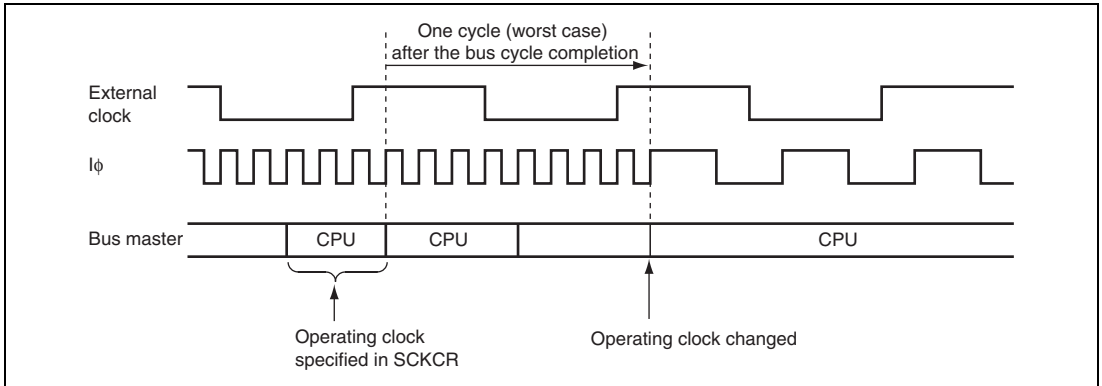
Figure 24.6 Clock Modification Timing
