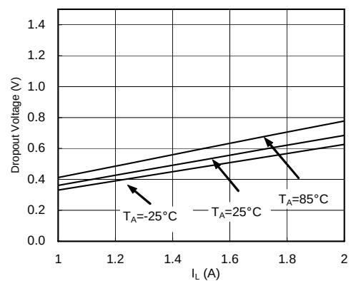
G954-18 Dropout Voltage vs. I L
