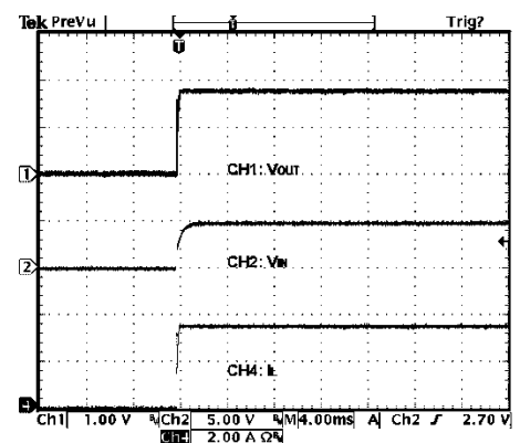
G954-18-Start-up
