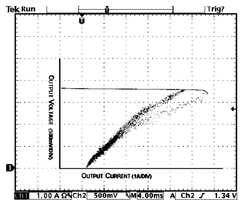
G954-18 Overcurrent Protection Characteristics
