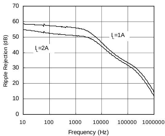
Ripple Rejection
