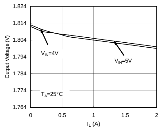
G954-18 Output Voltage vs. I L
