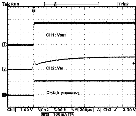
G954-18-Start-up
