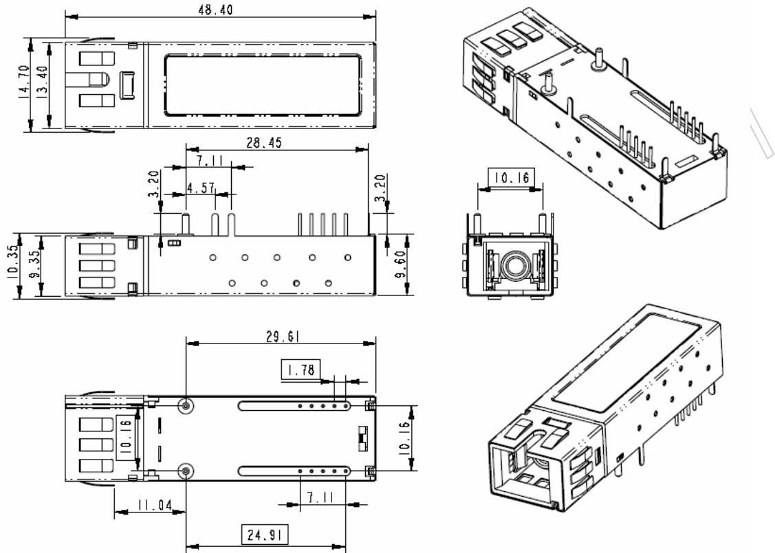
Figure 5 Mechanical Design Diagram
