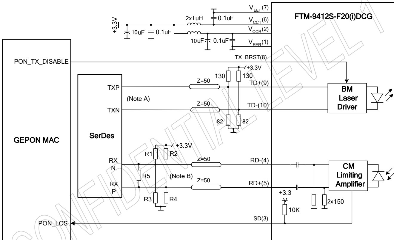
Figure 3 shows the recommended interface schemes for FTM-9412S-F20(i)DCG
