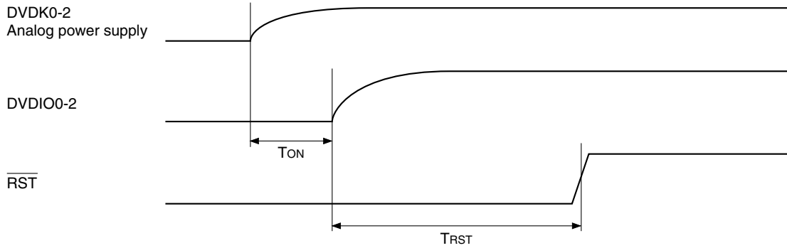
Fig. 4. Power-on Sequence
