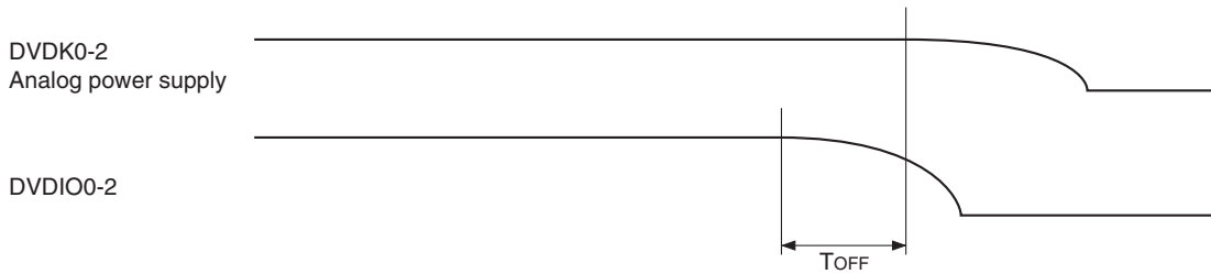
Fig. 5. Power-off Sequence
