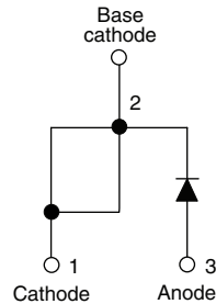
TO-247AC (modified)
