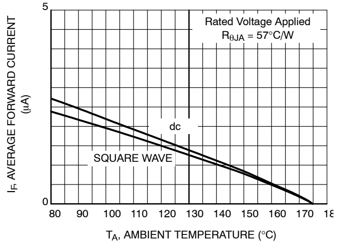
Figure 6. Typical Current Derating, Ambient
