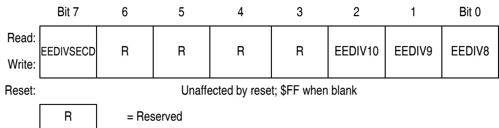
Figure 5-7. EEPROM-1 Divider Non-Volatile Register High (EE1DIVHNVR)
