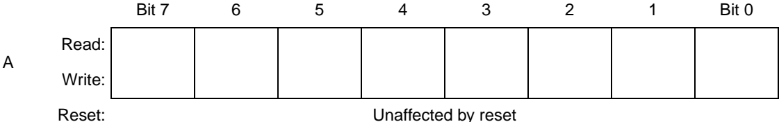
Figure 7-2. Accumulator (A)
