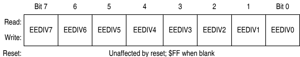
Figure 5-8. EEPROM-1 Divider Non-Volatile Register Low (EE1DIVLNVR)
