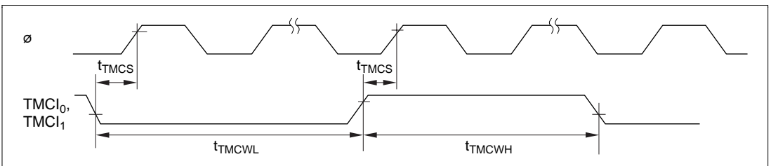
Figure 19.13 8-Bit Timer Clock Input Timing
