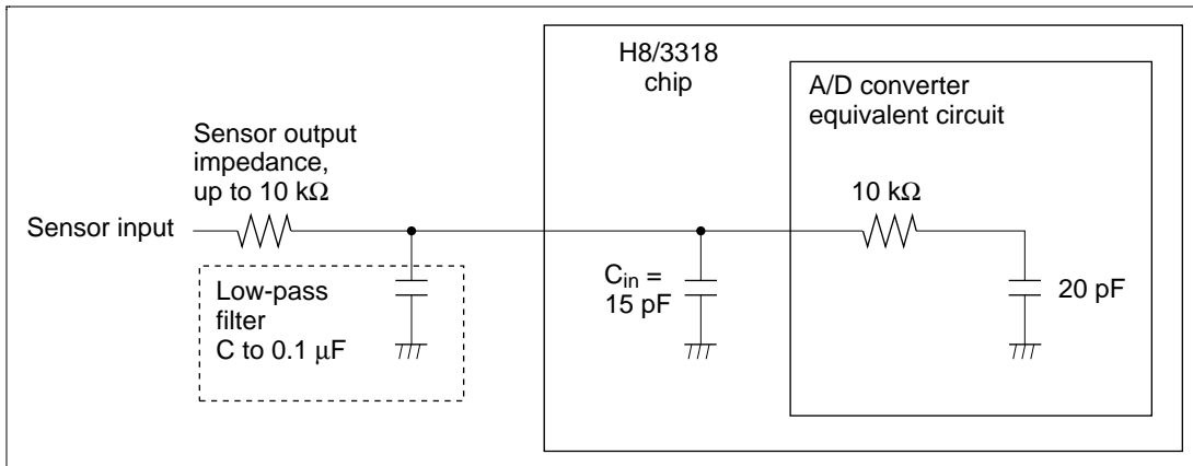
Figure 15.10 Example of Analog Input Circuit
