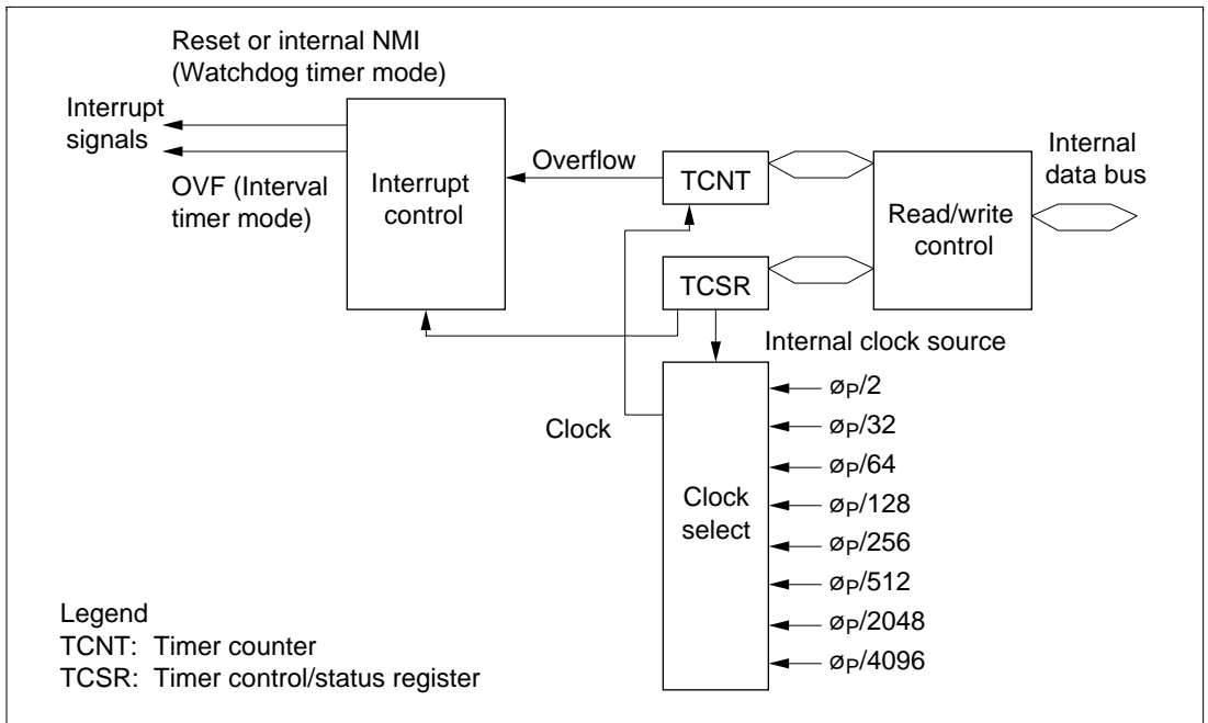
Figure 13.1 Block Diagram of Watchdog Timer
