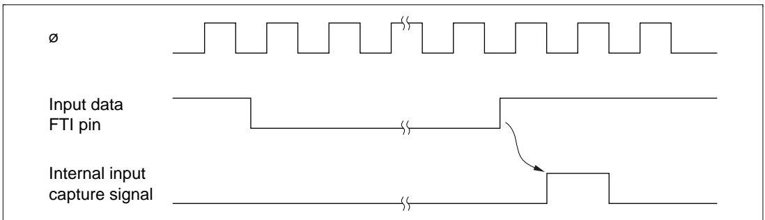
Figure 9.8 Input Capture Timing (Usual Case)
