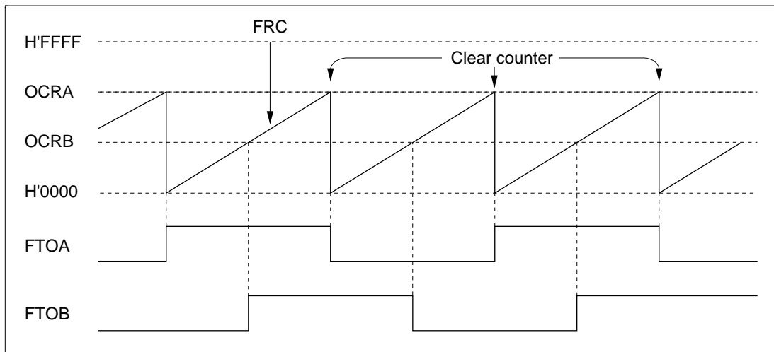
Figure 9.15 Square-Wave Output (Example)
