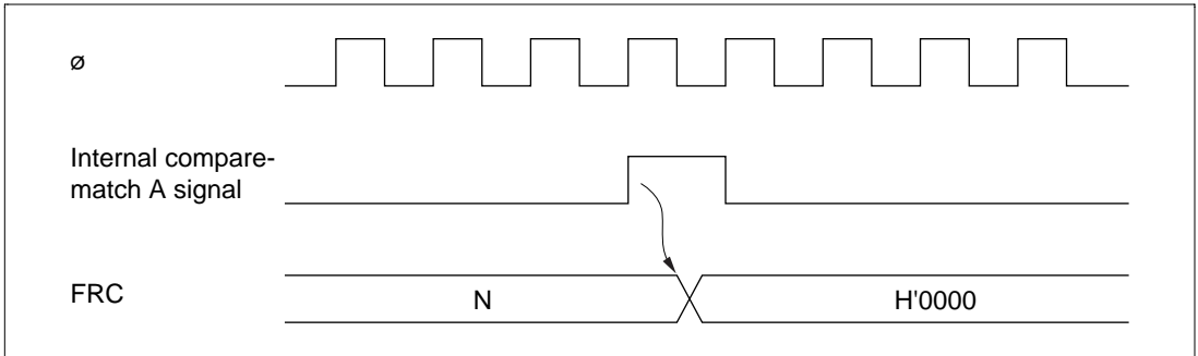
Figure 9.7 Clearing of FRC by Compare-Match A
