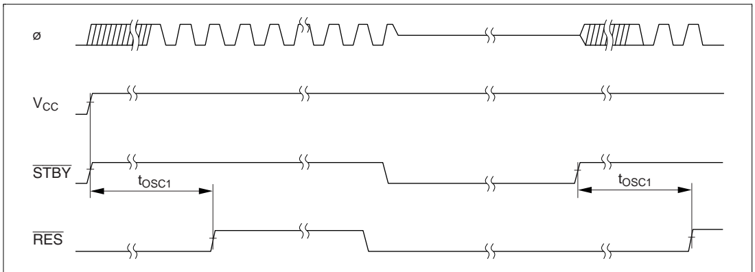
Figure 19.8 Clock Settling Timing
