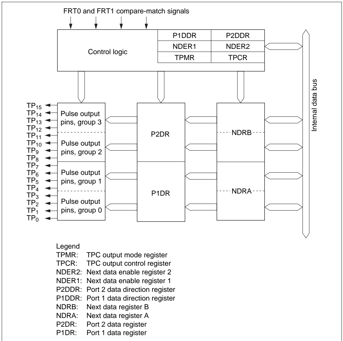
Figure 12.1 TPC Block Diagram
