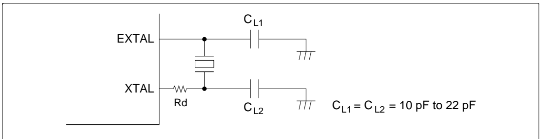
Figure 7.2 Connection of Crystal Oscillator (Example)
