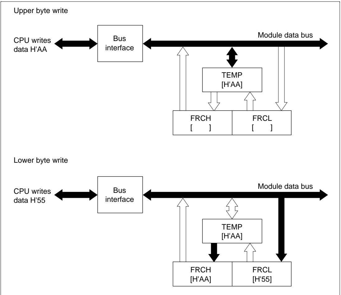
Figure 10.2a Write Access to FRC (When CPU Writes H'AA55)
