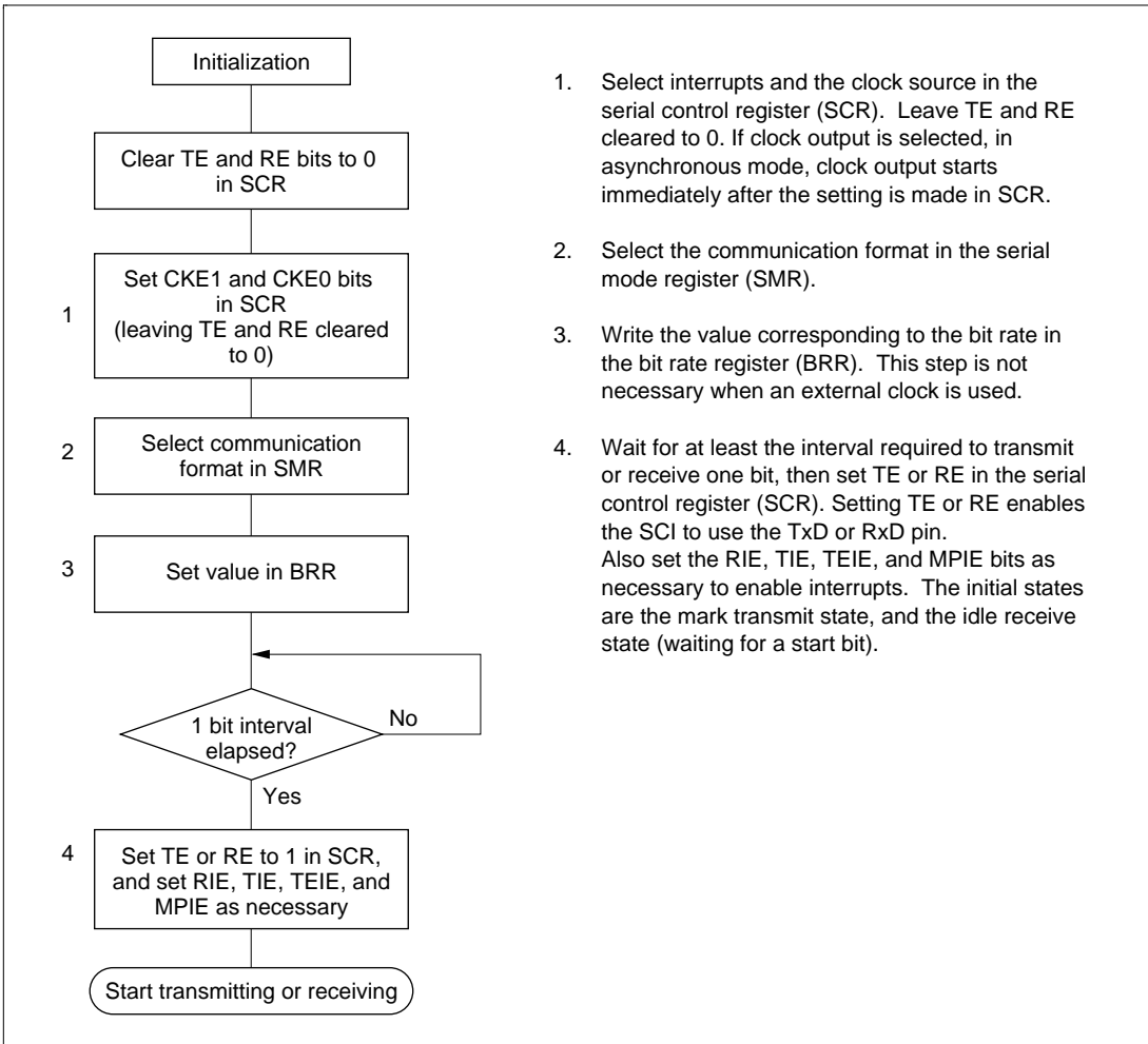
Figure 14.4 Sample Flowchart for SCI Initialization
