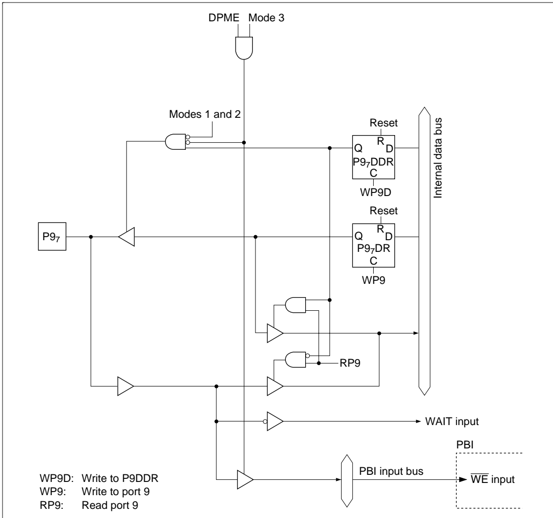
Figure C.9 (g) Port 9 Block Diagram (Pin P9 7 )
