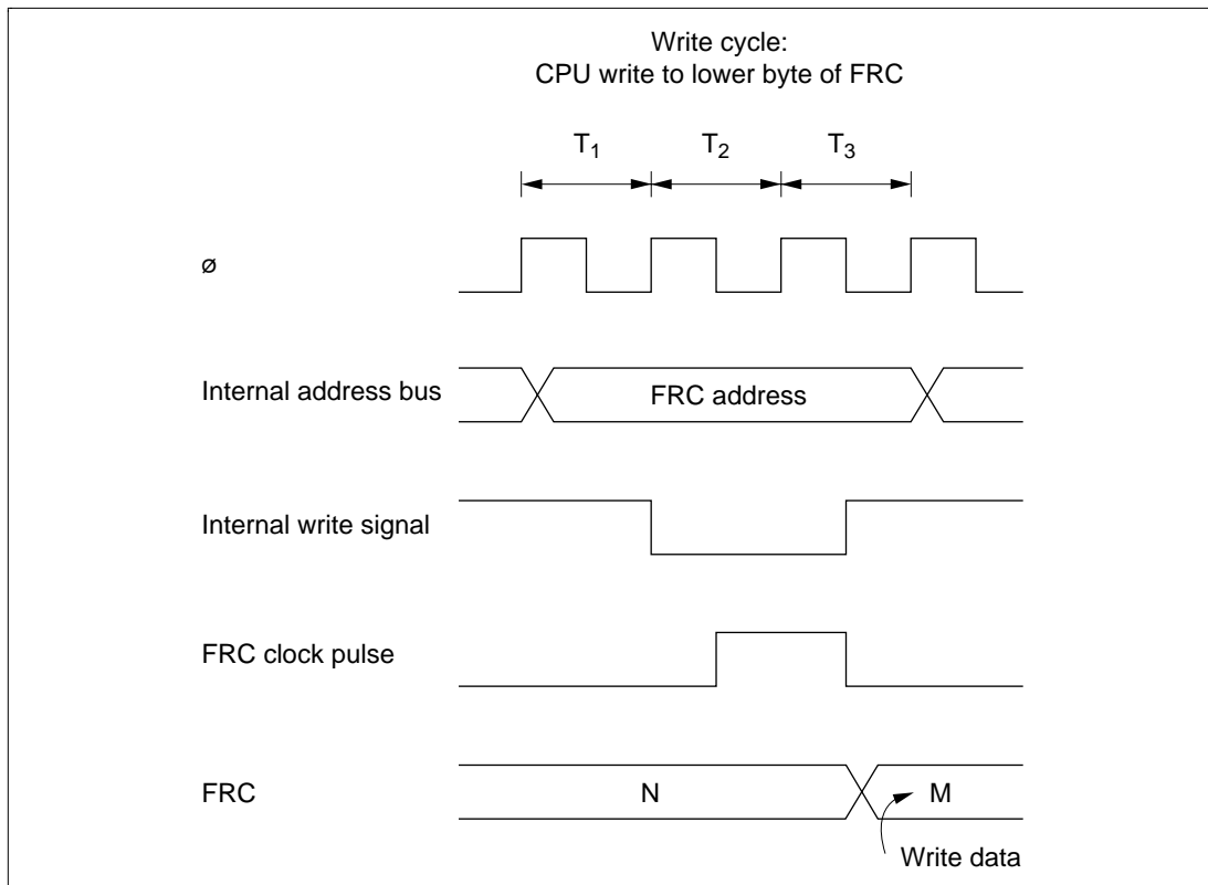
Figure 9.17 FRC Write-Increment Contention
