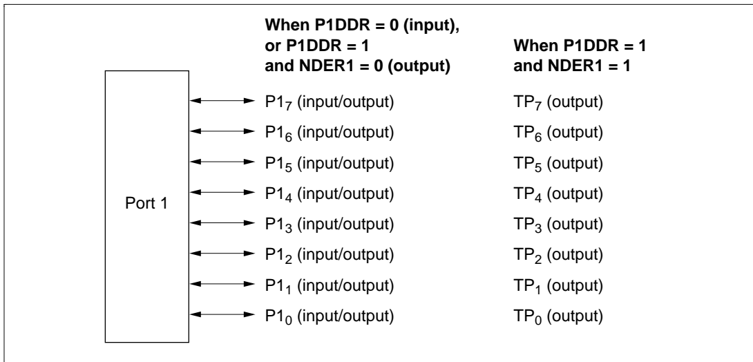
Figure 8.4 Pin Functions in Mode 3 (Port 1)
