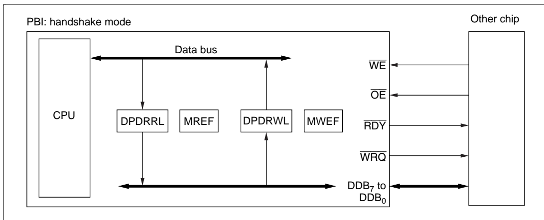
Figure 5.23 Transfers in Handshake Mode
