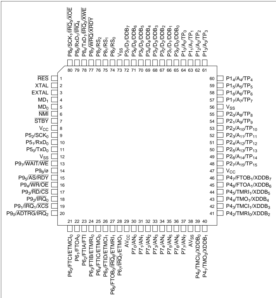
Figure 1.3 Pin Arrangement (FP-80A and TFP-80C, Top View)
