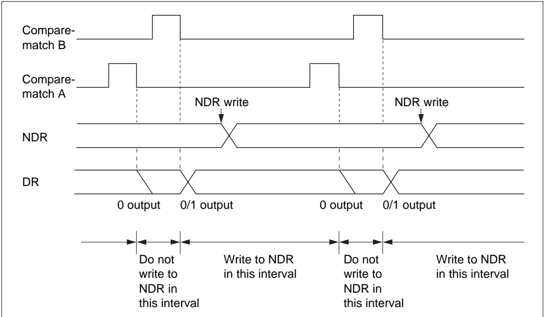
Figure 12.9 Non-Overlapping Operation and NDR Write Timing
