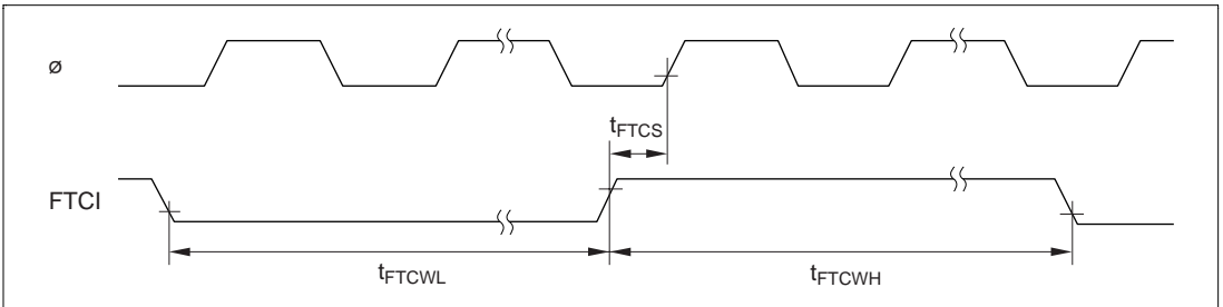
Figure 19.11 External Clock Input Timing for Free-Running Timer
