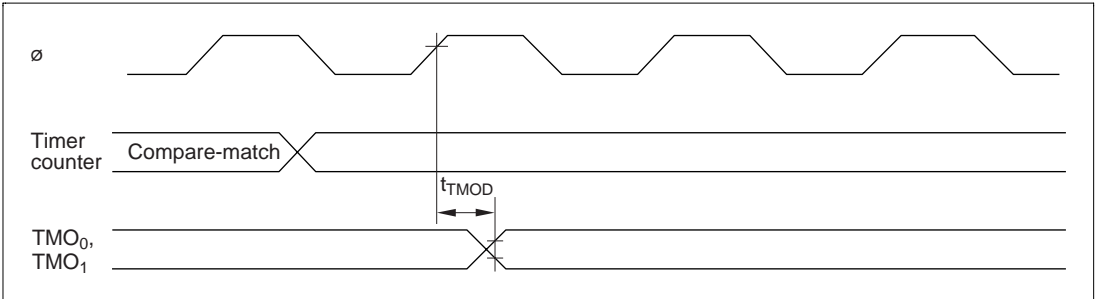
Figure 19.12 8-Bit Timer Output Timing
