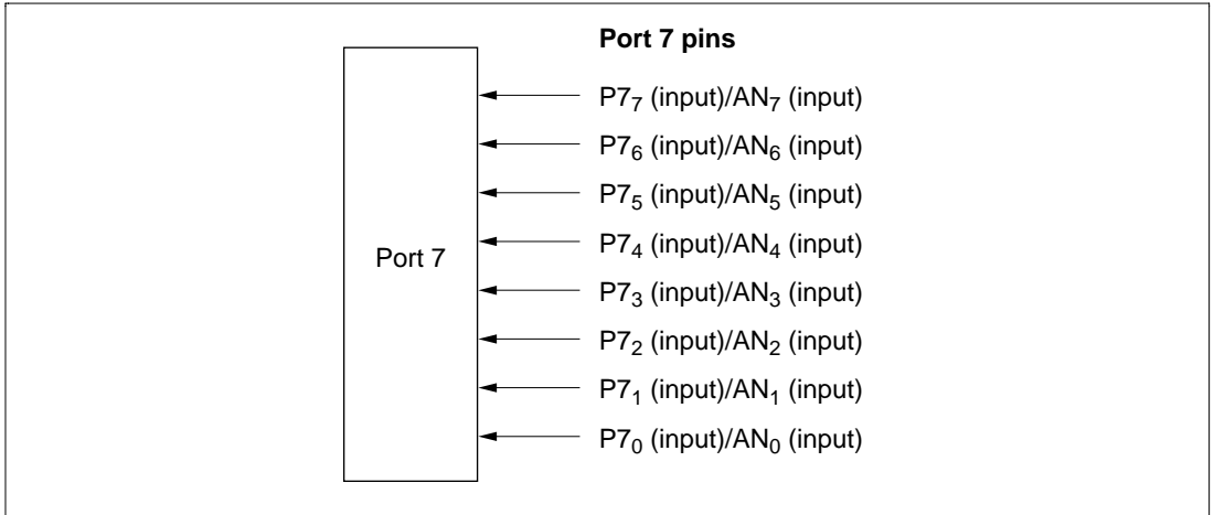
Figure 8.17 Port 7 Pin Configuration
