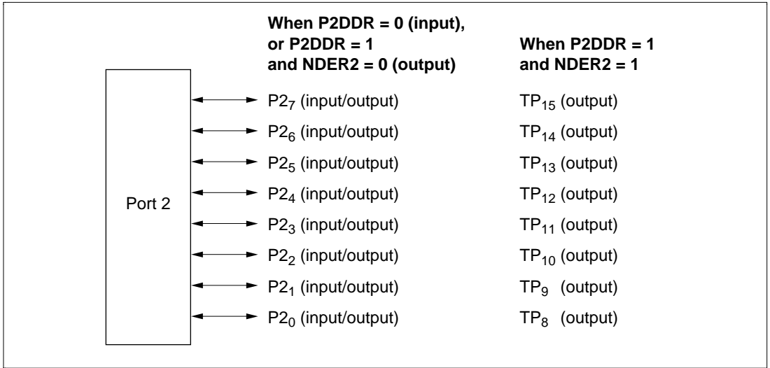
Figure 8.8 Pin Functions in Mode 3 (Port 2)
