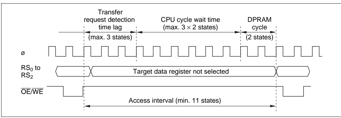
Figure 5.32 Buffer Query Mode Address Write to Data Read Access Interval
