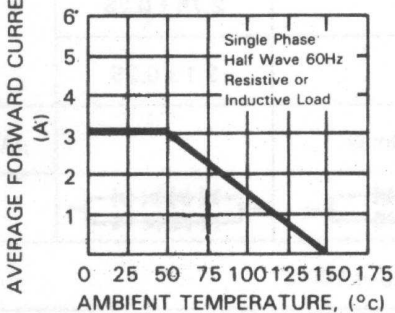
FIG. 5 - TYPICAL FORWARD CURRENT DERATING CURVE
