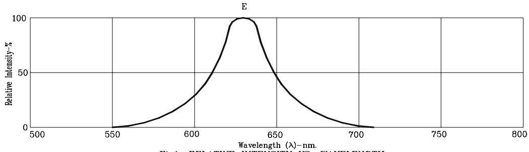
Fig1. RELATIVE INTENSITY VS. WAVELENGTH
