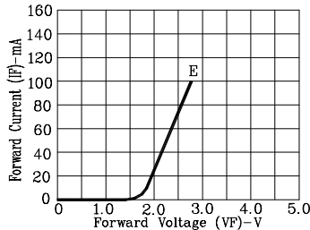
Fig3. FORWARD CURRENT VS. FORWARD VOLTAGE
