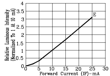
Fig4. RELATIVE LUMINOUS INTENSITY VS. FORWARD CURRENT
