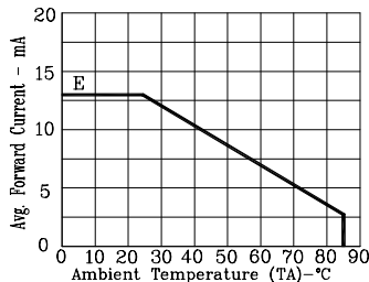
Fig5. MAX. AVERAGE FORWARD CURRENT VS. AMBIENT TEMPERATURE.
