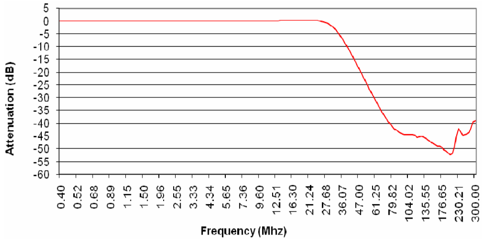
Figure 7. FMS6303 1080i HD Frequency Response
