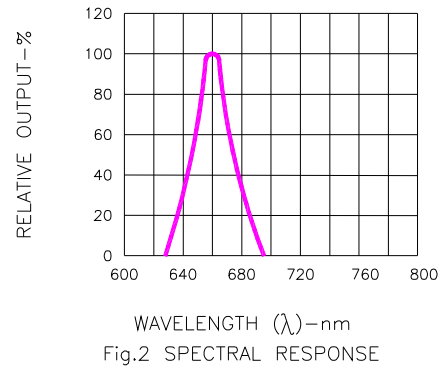
Fig.2 SPECTRAL RESPONSE
