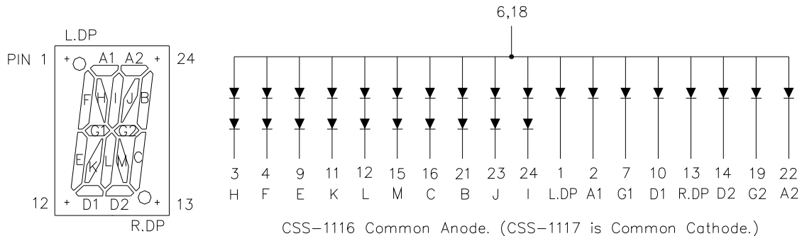
CSS-1116 Common Anode. (CSS-1117 is Common Cathode.) NO. 5, 8, 17, 20 No Pin.
