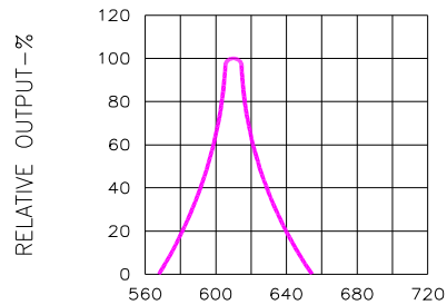
Fig.2 SPECTRAL RESPONSE
