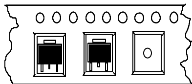
Feed Direction TO-252, TO-263 Package Orientation
