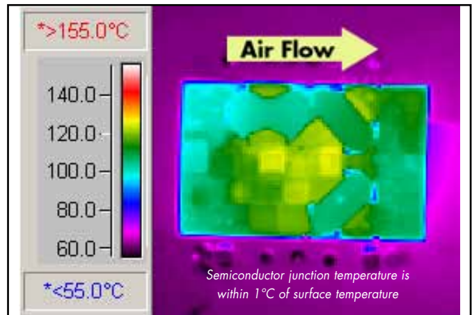
Figure 10: Thermal plot of converter at 24 amp load current with 55°C air flowing at the rate of 200 LFM. Air is flowing across the converter from input to output (24V input).
