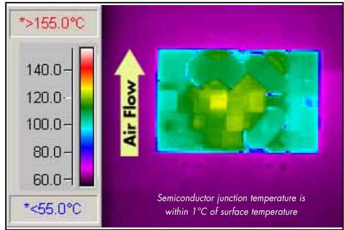
Figure 8: Thermal plot of converter at 25 amp load current with 55°C air flowing at the rate of 200 LFM. Air is flowing across the converter from pin 3 to pin 1 (48V input).
