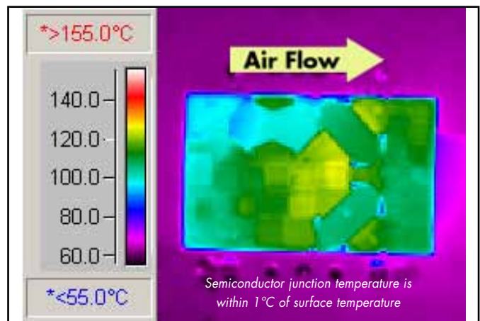
Figure 12: Thermal plot of converter at 24 amp load current with 55°C air flowing at the rate of 200 LFM. Air is flowing across the converter from input to output (48V input).
