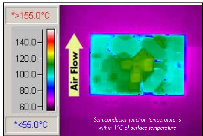
Figure 6: Thermal plot of converter at 25 amp load current with 55°C air flowing at the rate of 200 LFM. Air is flowing across the converter from pin 3 to pin 1 (24V input).
