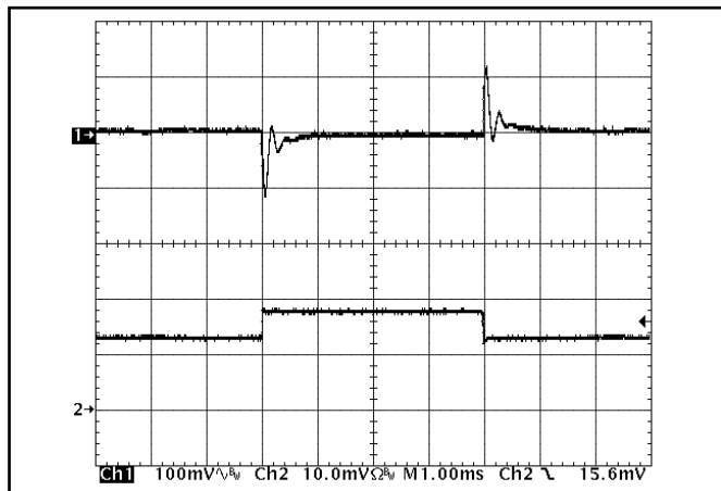
Figure 16: Output voltage response to step-change in load current (50%-75%-50% of I_{out(max)} ; di/dt = 5A/\mu s ). Load cap: 470 \mu F , 30 m \Omega ESR tantalum cap and 1 \mu F ceramic cap. Ch 1: V_{out} (100mV/div), Ch 2: I_{out} (10A/div).
