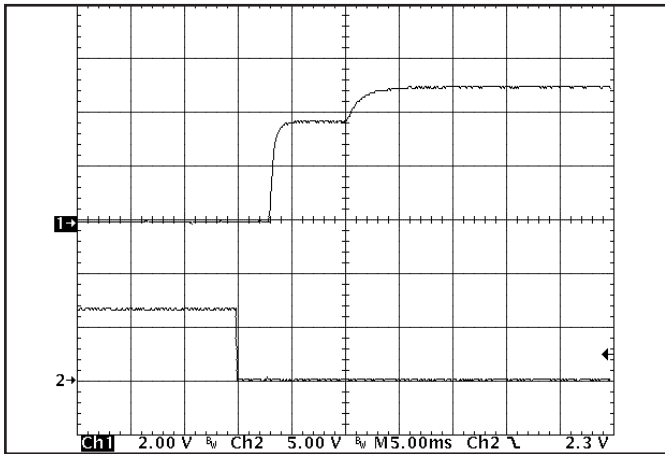
Figure 13: Turn-on transient at full load (resistive load) (5 ms/div). Input voltage pre-applied. Ch 1: Vout (2V/div). Ch 2: ON/OFF input (5V/div).
