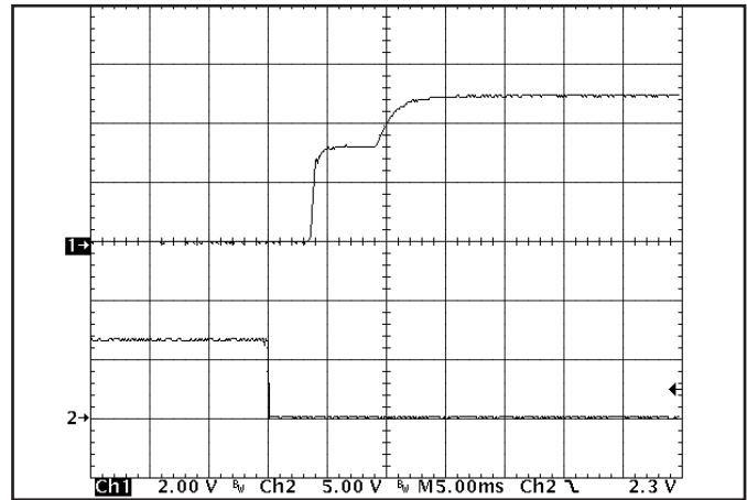
Figure 14: Turn-on transient at zero load (5 ms/div). Ch 1: Vout (2V/div). Ch 2: ON/OFF input (5V/div).
