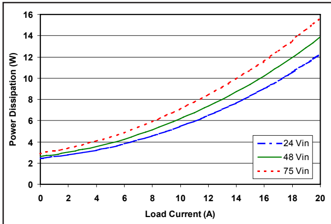
Figure 3: Power dissipation at nominal output voltage vs. load current for 24V, 48V and 75V input at 25°C.
