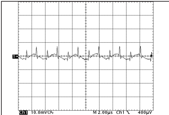
Figure 19: Input reflected ripple current, i_s , through a 10\ \mu\text{H} source inductor at nominal input voltage and rated load current (20 mA/div). See Figure 17.
