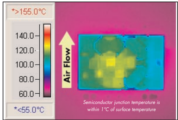
Figure 8: Thermal plot of converter at 17 amp load current with 55°C air flowing at the rate of 200 LFM. Air is flowing across the converter sideways from pin 3 to pin 1 (48V input).
