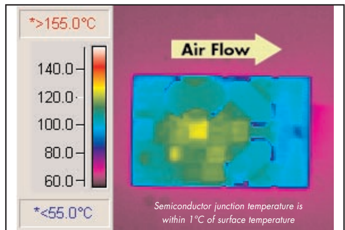
Figure 12: Thermal plot of converter at 17 amp load current with 55°C air flowing at the rate of 200 LFM. Air is flowing across the converter from input to output (48V input).
