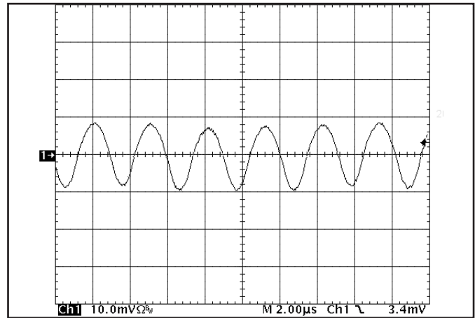
Figure 18: Input Terminal Ripple Current, i_c , at full rated output current and nominal input voltage with 10\ \mu\text{H} source impedance and 47\ \mu\text{F} electrolytic capacitor (20 mA/div). See Figure 17.
