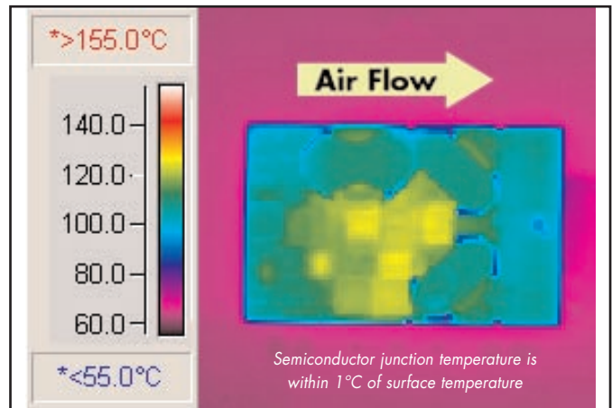
Figure 10: Thermal plot of converter at 19 amp load current with 55°C air flowing at the rate of 200 LFM. Air is flowing across the converter from input to output (24V input).
