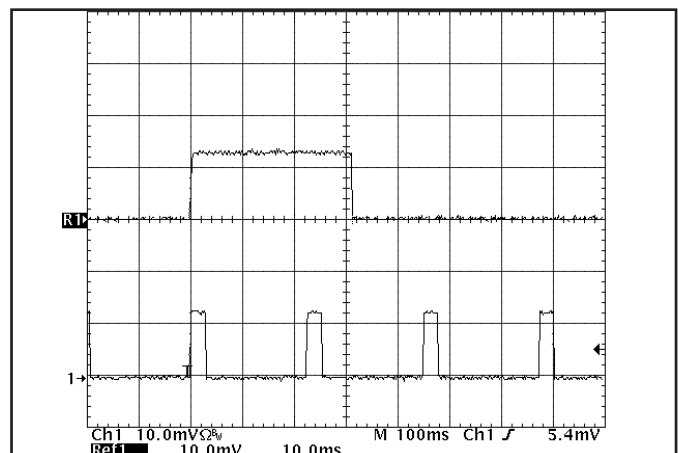
Figure 22: Load current (20A/div) as a function of time when the converter attempts to turn on into a 10\ \text{m}\Omega short circuit. Top trace (10ms/div) is an expansion of the on-time portion of the bottom trace.
