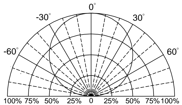
Fig.6 Directivity Radiation
