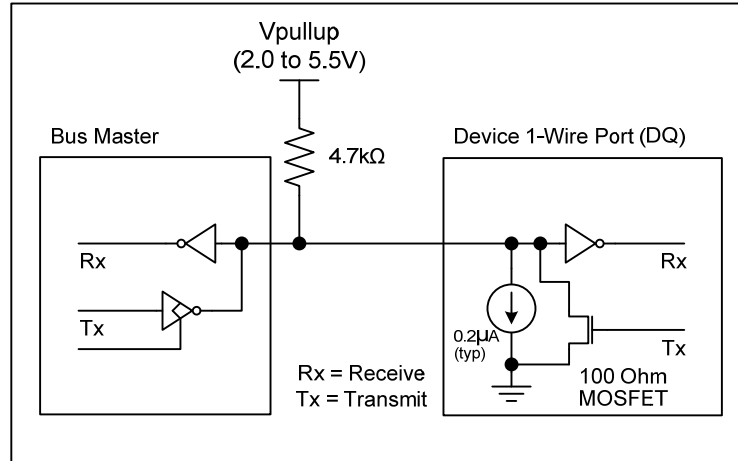
Figure 9. 1-Wire Bus Interface Circuitry
