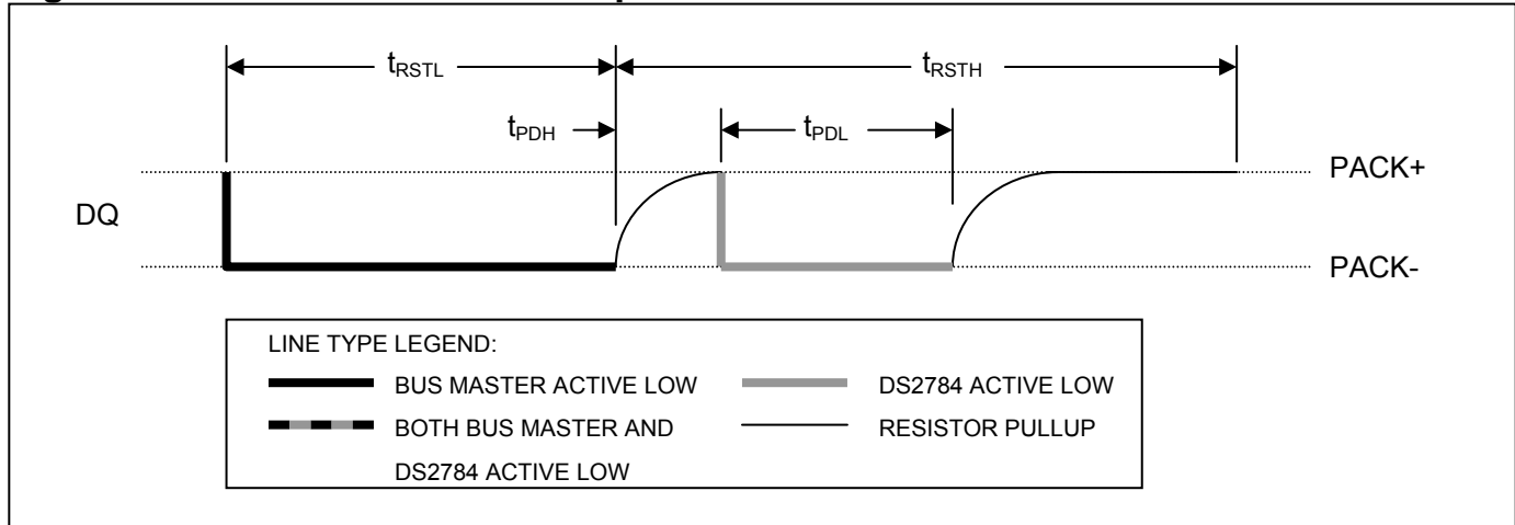
Figure 14. 1-Wire Initialization Sequence
