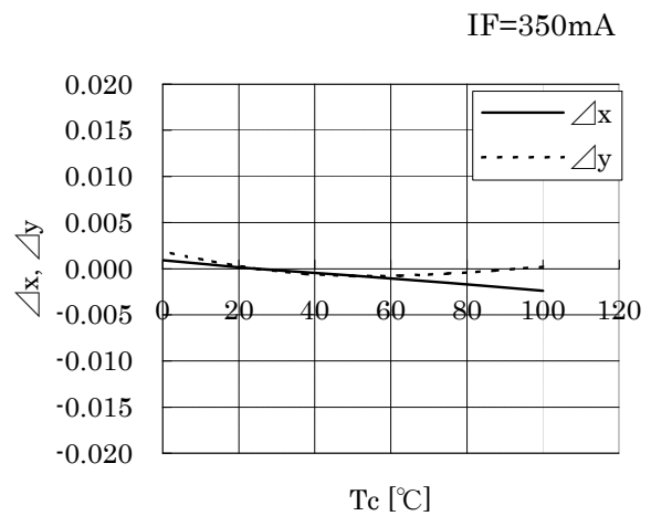
Case Temperature vs. Chromaticity Coordinate
