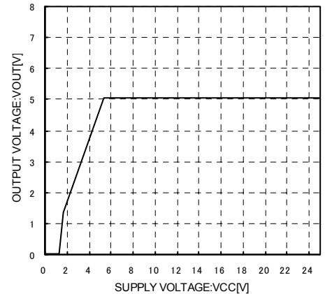
Fig.15 Input Stability (Io=2A)
