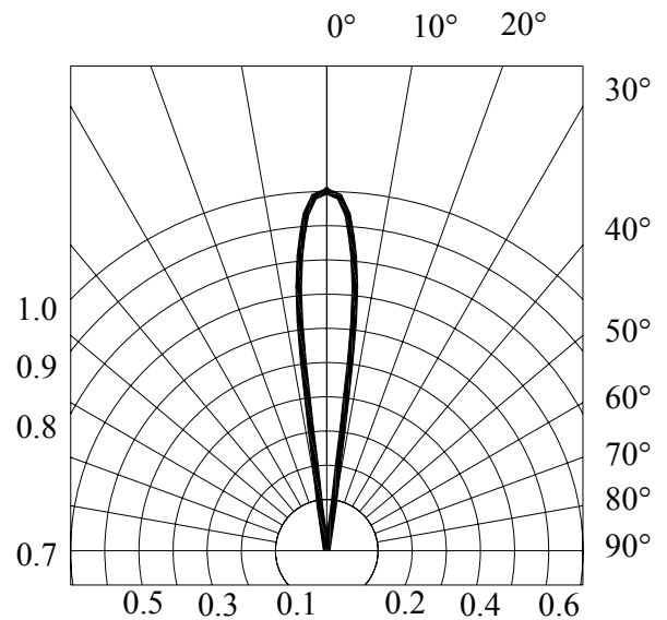
RADIATION DIAGRAM
