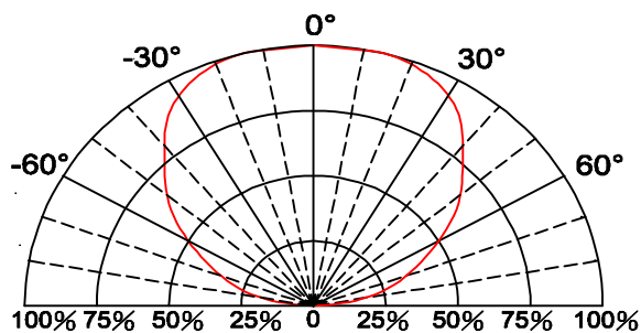
Fig.5 Directive Radiation
