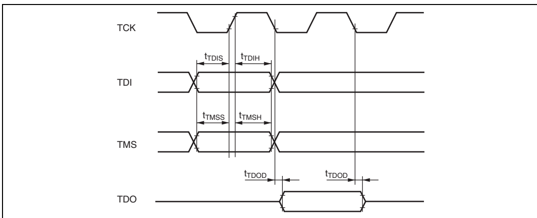
Figure 26.23 Boundary Scan Data Transmission Timing
