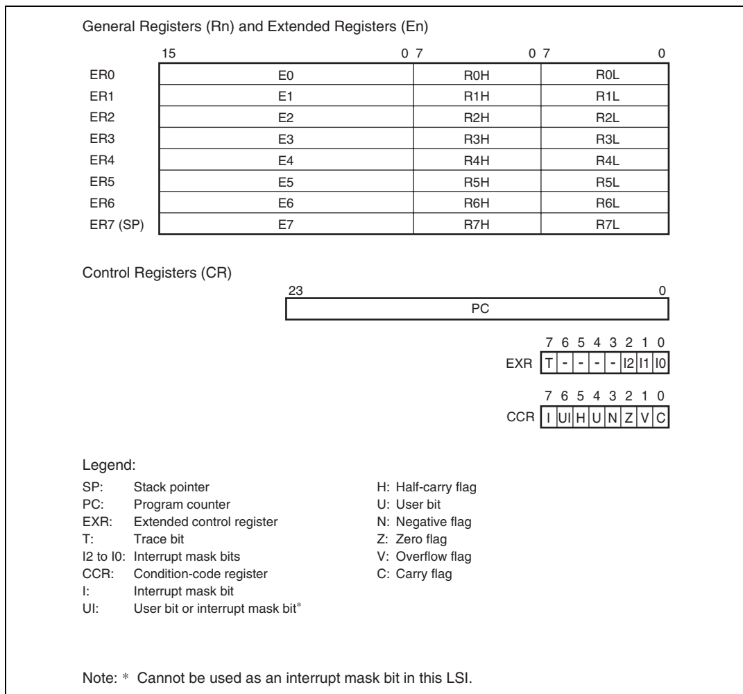
Figure 2.6 CPU Registers
