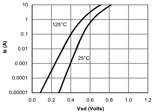
Figure 6: Body-Diode Characteristics
