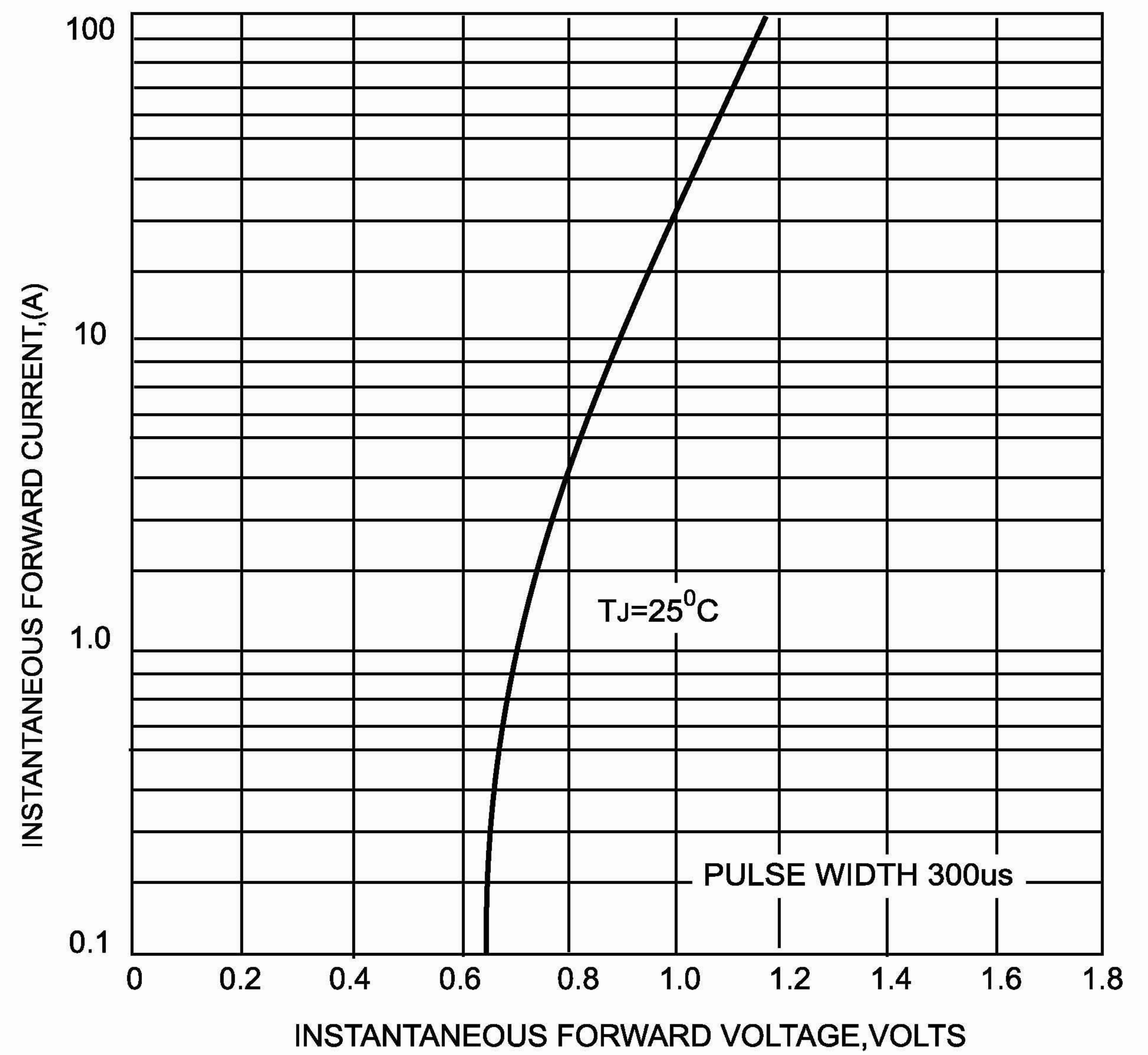
FIG.4- TYPICAL FORWARD CHARACTERISTICS
