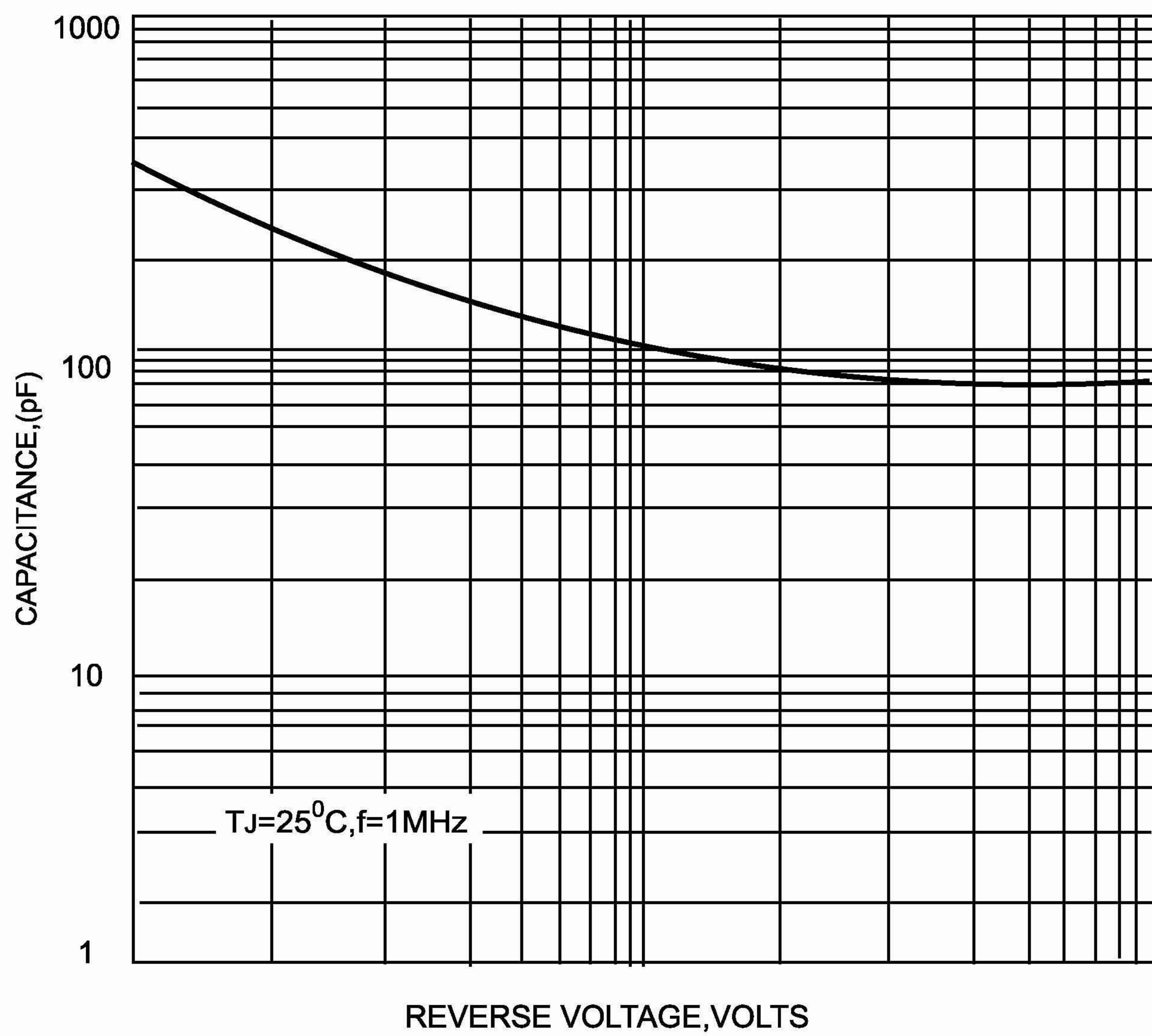
FIG.3- TYPICAL JUNCTION CAPACITANCE
