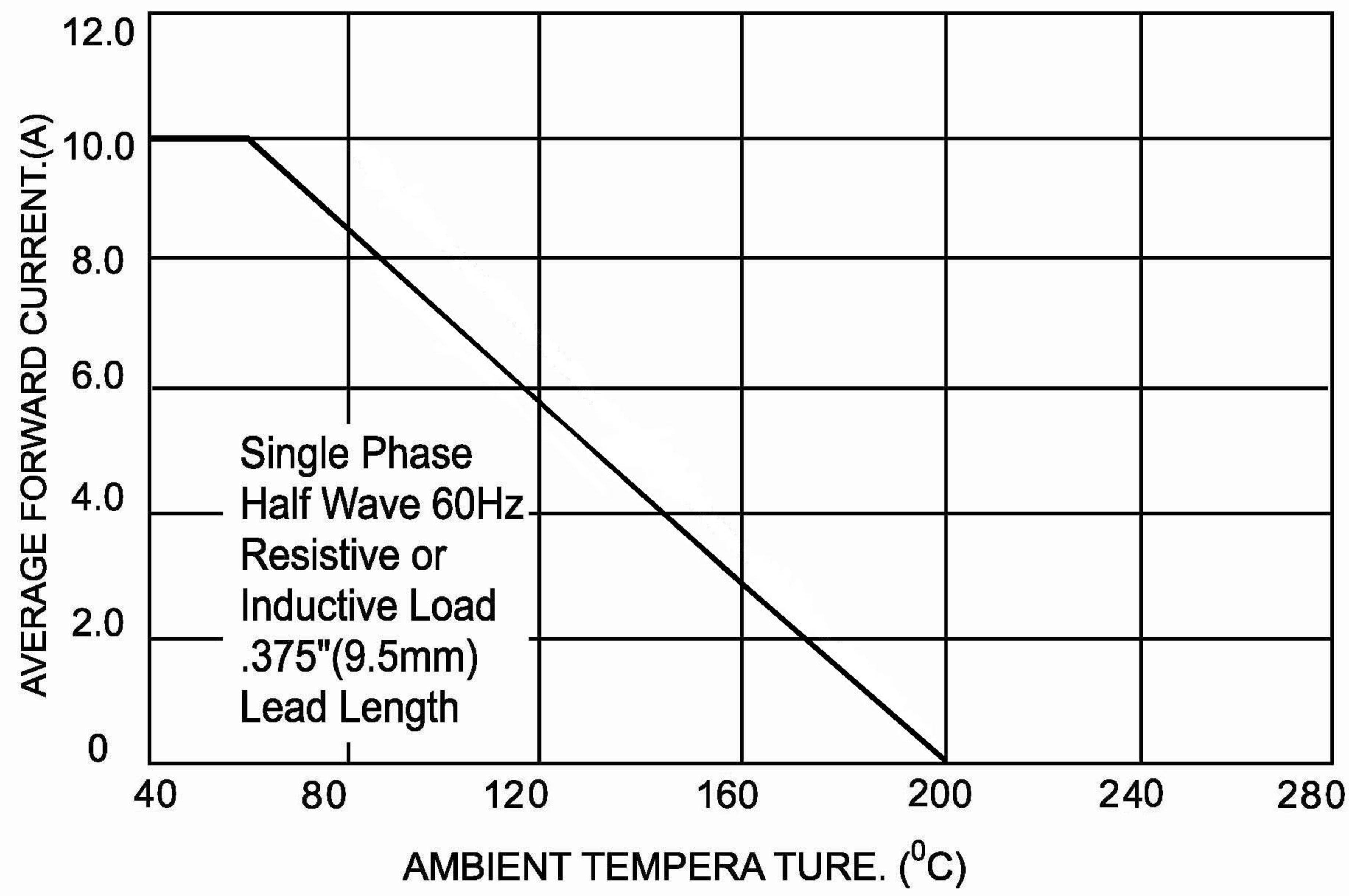
FIG.1- FORWARD CURRENT DERATING CURVE
