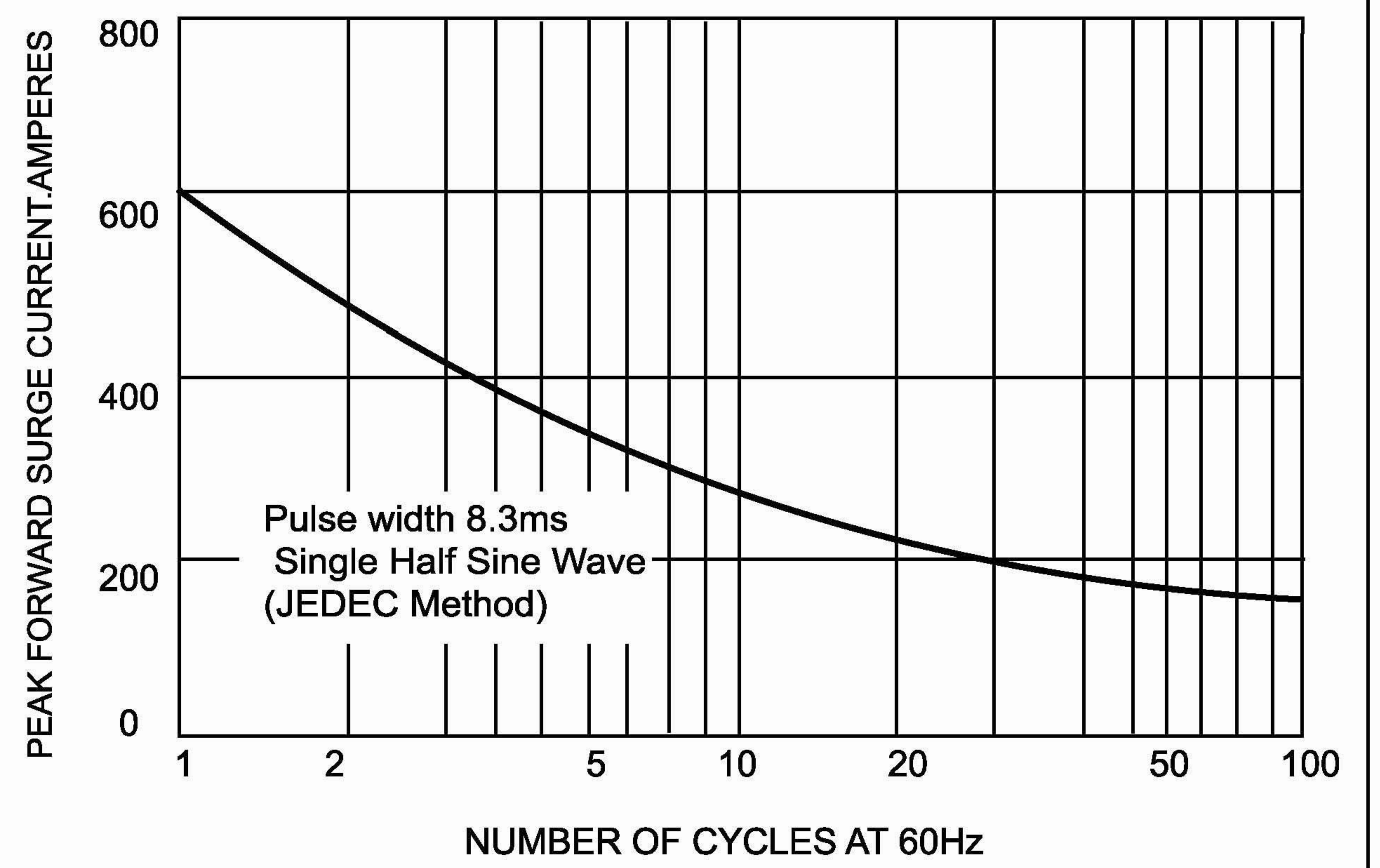
FIG.2- MAXIMUM NON-REPETITIVE SURGE CURRENT
