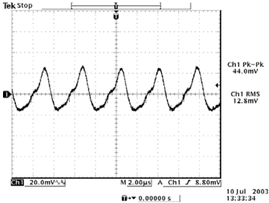
10 Vdc input, 3.3 Vdc output
