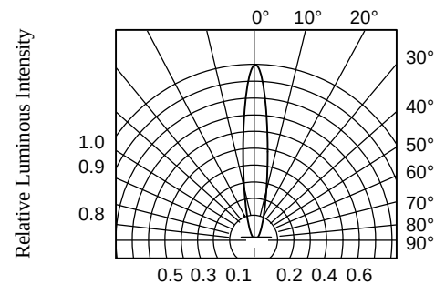
FIG.6 RADIATION DIAGRAM
