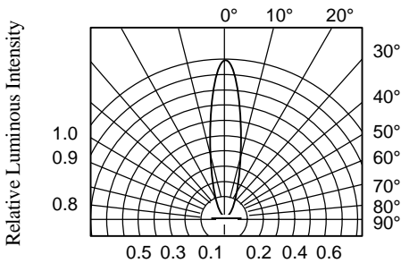
FIG.6 RADIATION DIAGRAM
