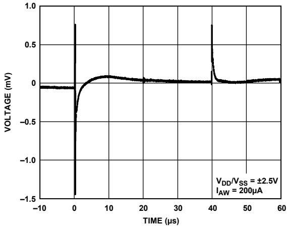
Figure 19. Digital Feedthrough
