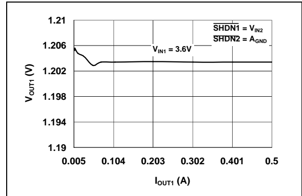
FIGURE 2-10: V_{OUT1} vs. I_{OUT1} ( V_{OUT1} = 1.2\text{V} ).
