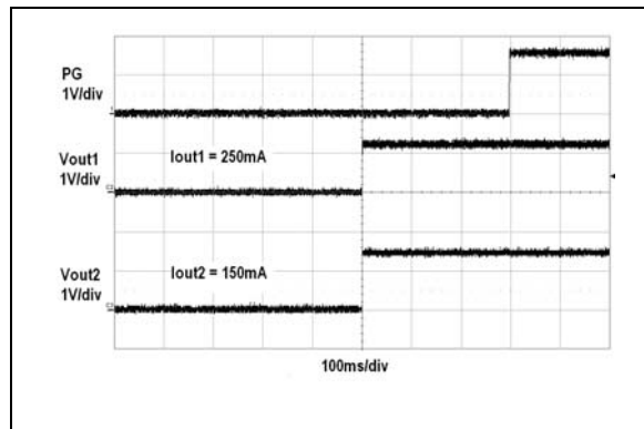
FIGURE 2-40: Power-Good Output Timing.
