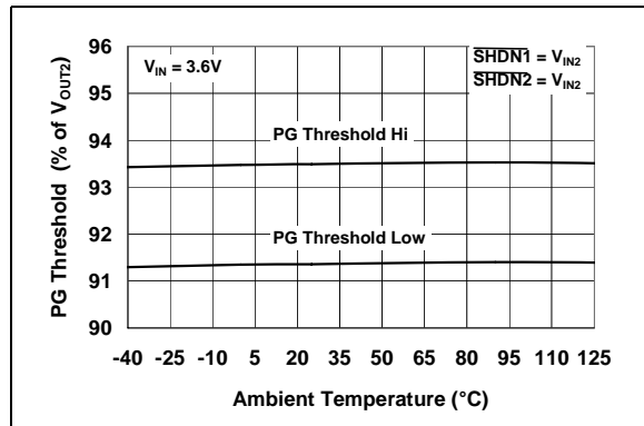
FIGURE 2-30: PG Threshold Voltage vs. Ambient Temperature.
