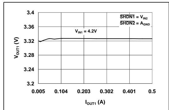
FIGURE 2-12: V_{OUT1} vs. I_{OUT1} ( V_{OUT1} = 3.3\text{V} ).
