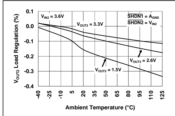
FIGURE 2-28: V_{OUT2} Load Regulation vs. Ambient Temperature.
