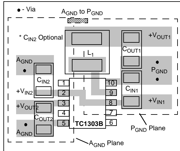
FIGURE 5-1: Component Placement, Fixed 10-Pin MSOP.
