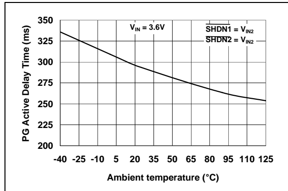
FIGURE 2-29: PG Active Delay Time-out vs. Ambient Temperature.
