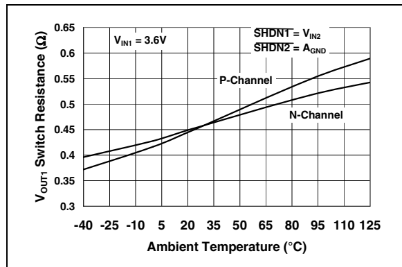
FIGURE 2-17: Buck Regulator Switch Resistance vs. Ambient Temperature.
