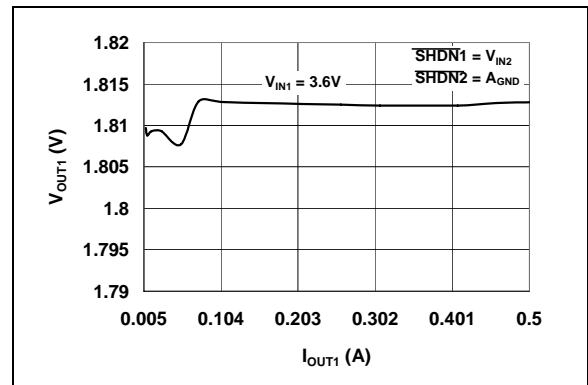
FIGURE 2-11: V_{OUT1} vs. I_{OUT1} ( V_{OUT1} = 1.8\text{V} ).
