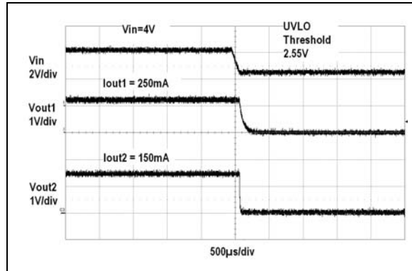
FIGURE 2-39: V_{OUT1} and V_{OUT2} Shutdown Waveforms.
