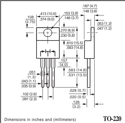
TO-220
