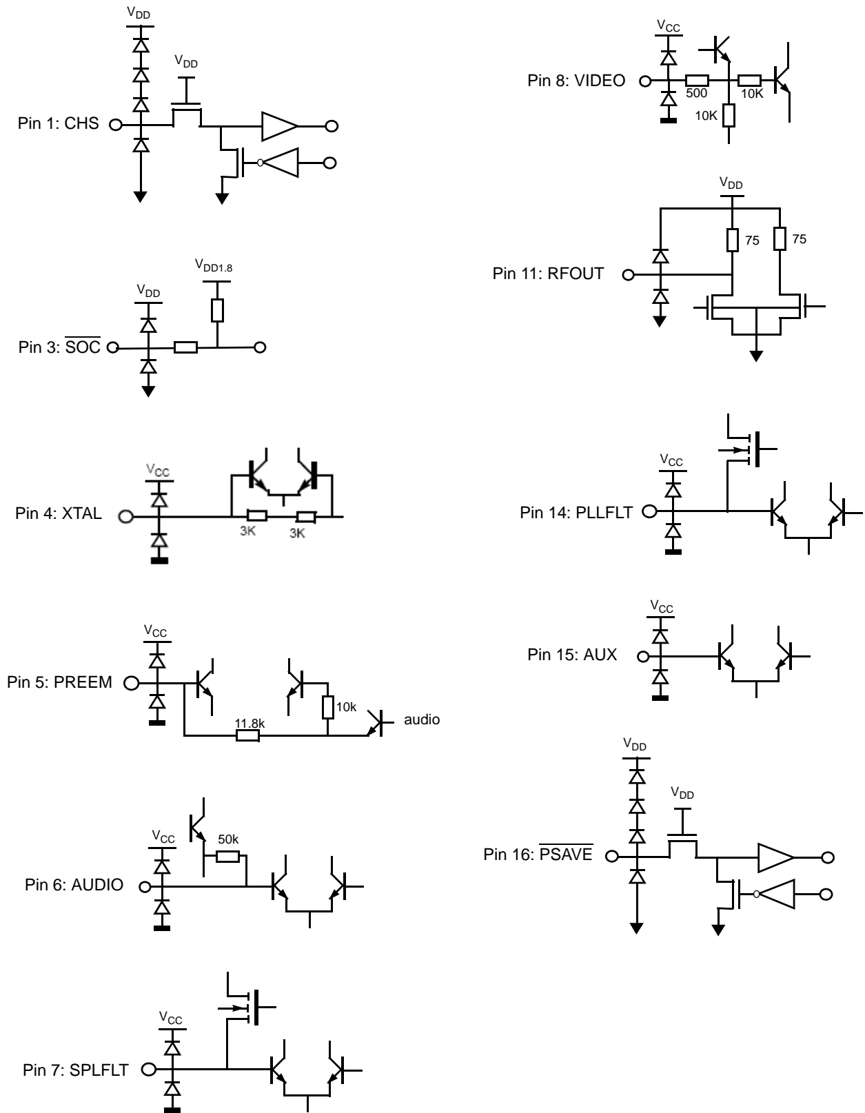
Figure 3. Pin Schematics
